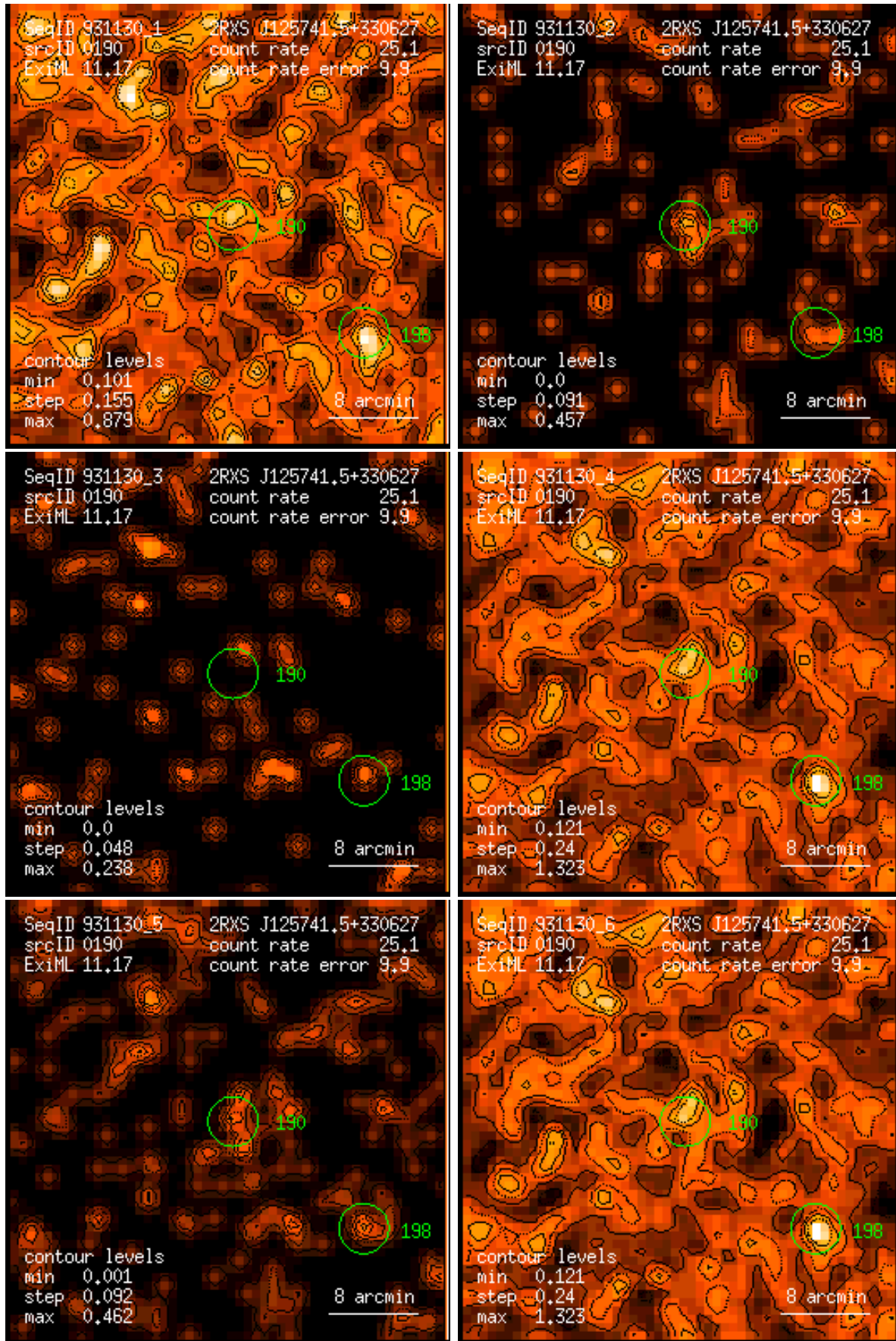
Figure 190: RASS 931130: detection 0190: band rate images, Gaussian filter: (1) PSPC channels 11 – 41, (2) 52 – 90, (3) 91 – 201, (4) 11 – 235, (5) 52 – 201, (6) 11 – 201. Broad band rates in counts/ks. Band rate contour levels in counts/ks/arcmin 2 .
