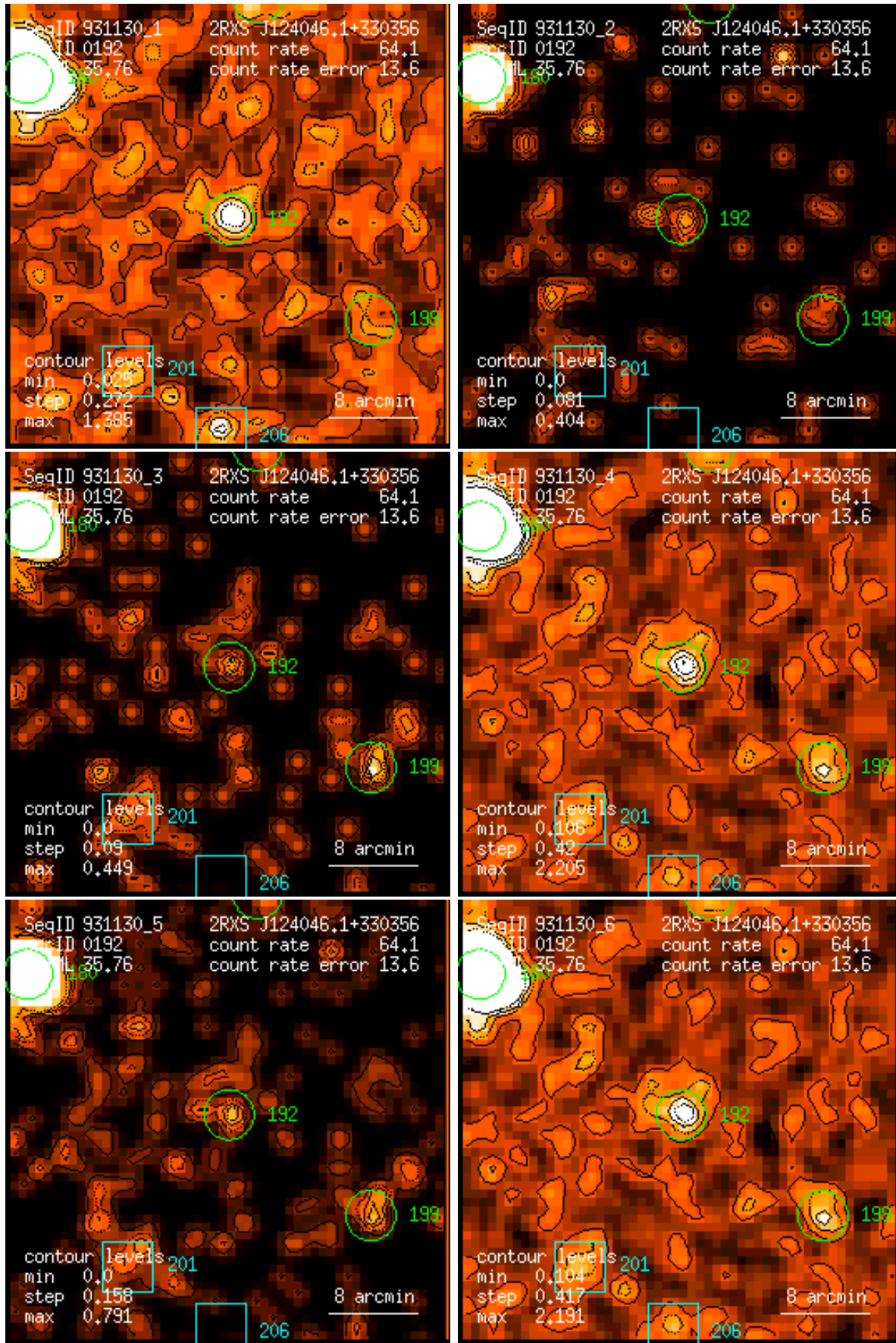
Figure 192: RASS 931130: detection 0192: band rate images, Gaussian filter: (1) PSPC channels 11 – 41, (2) 52 – 90, (3) 91 – 201, (4) 11 – 235, (5) 52 – 201, (6) 11 – 201. Broad band rates in counts/ks. Band rate contour levels in counts/ks/arcmin 2 .
