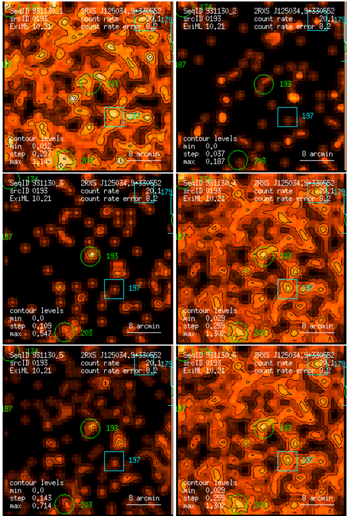
Figure 193: RASS 931130: detection 0193: band rate images, Gaussian filter: (1) PSPC channels 11 – 41, (2) 52 – 90, (3) 91 – 201, (4) 11 – 235, (5) 52 – 201, (6) 11 – 201. Broad band rates in counts/ks. Band rate contour levels in counts/ks/arcmin 2 .
