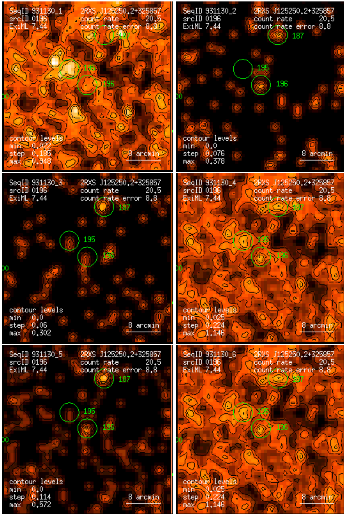
Figure 196: RASS 931130: detection 0196: band rate images, Gaussian filter: (1) PSPC channels 11 – 41, (2) 52 – 90, (3) 91 – 201, (4) 11 – 235, (5) 52 – 201, (6) 11 – 201. Broad band rates in counts/ks. Band rate contour levels in counts/ks/arcmin 2 .
