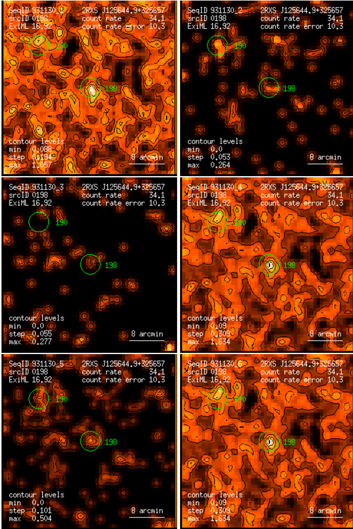
Figure 198: RASS 931130: detection 0198: band rate images, Gaussian filter: (1) PSPC channels 11 – 41, (2) 52 – 90, (3) 91 – 201, (4) 11 – 235, (5) 52 – 201, (6) 11 – 201. Broad band rates in counts/ks. Band rate contour levels in counts/ks/arcmin 2 .
