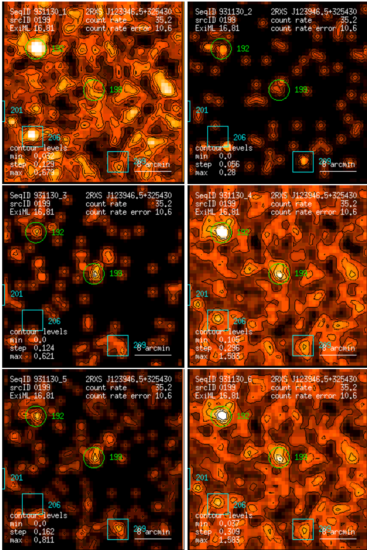
Figure 199: RASS 931130: detection 0199: band rate images, Gaussian filter: (1) PSPC channels 11 – 41, (2) 52 – 90, (3) 91 – 201, (4) 11 – 235, (5) 52 – 201, (6) 11 – 201. Broad band rates in counts/ks. Band rate contour levels in counts/ks/arcmin 2 .
