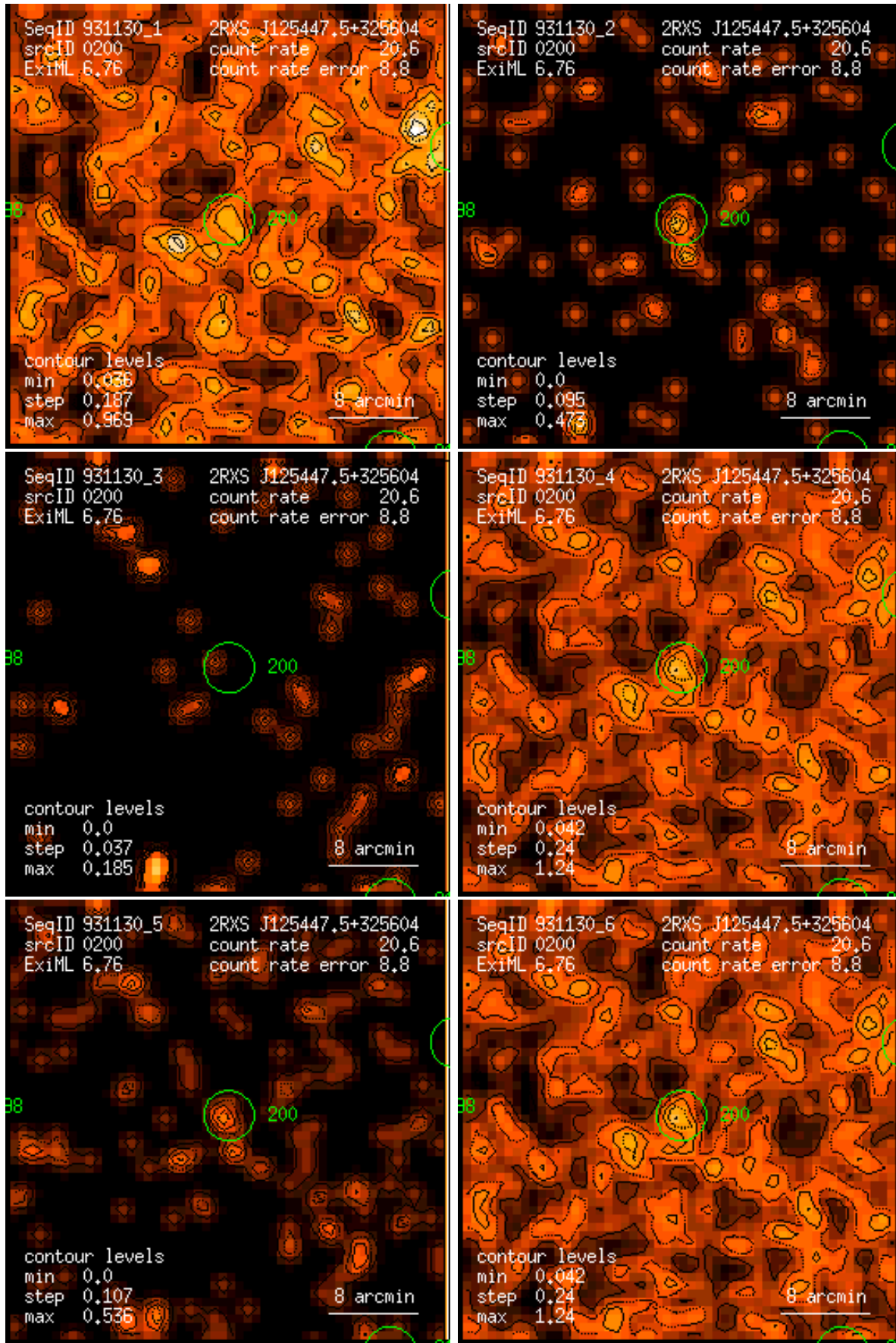
Figure 200: RASS 931130: detection 0200: band rate images, Gaussian filter: (1) PSPC channels 11 – 41, (2) 52 – 90, (3) 91 – 201, (4) 11 – 235, (5) 52 – 201, (6) 11 – 201. Broad band rates in counts/ks. Band rate contour levels in counts/ks/arcmin 2 .
