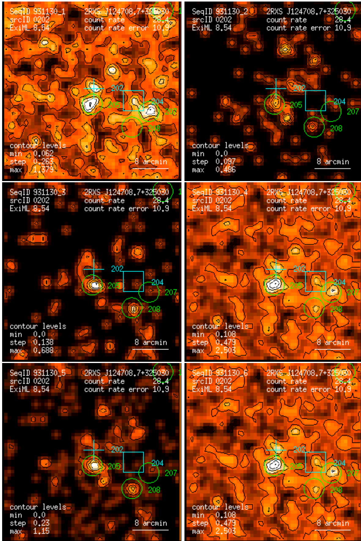
Figure 202: RASS 931130: detection 0202: band rate images, Gaussian filter: (1) PSPC channels 11 – 41, (2) 52 – 90, (3) 91 – 201, (4) 11 – 235, (5) 52 – 201, (6) 11 – 201. Broad band rates in counts/ks. Band rate contour levels in counts/ks/arcmin 2 .
