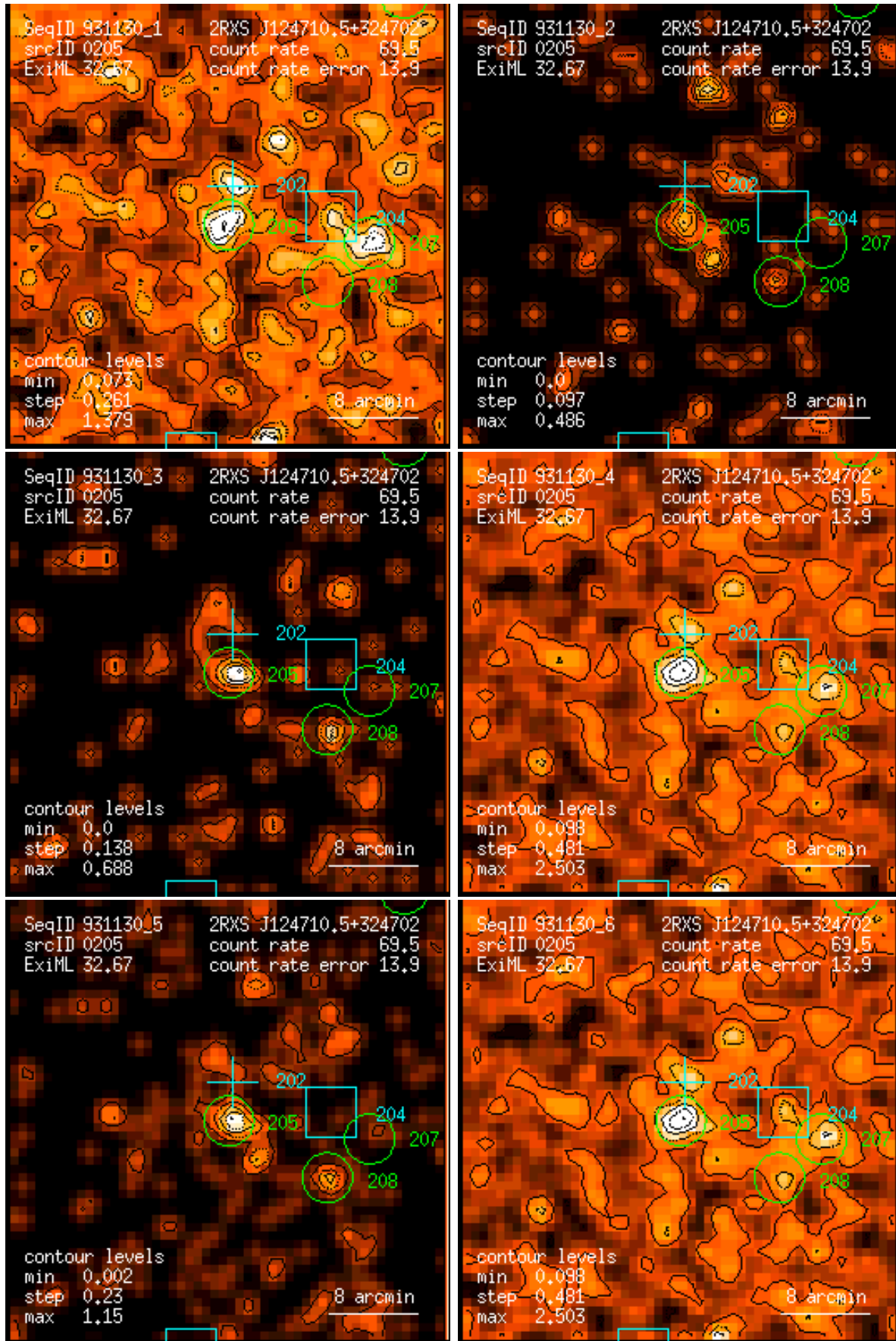
Figure 205: RASS 931130: detection 0205: band rate images, Gaussian filter: (1) PSPC channels 11 – 41, (2) 52 – 90, (3) 91 – 201, (4) 11 – 235, (5) 52 – 201, (6) 11 – 201. Broad band rates in counts/ks. Band rate contour levels in counts/ks/arcmin 2 .
