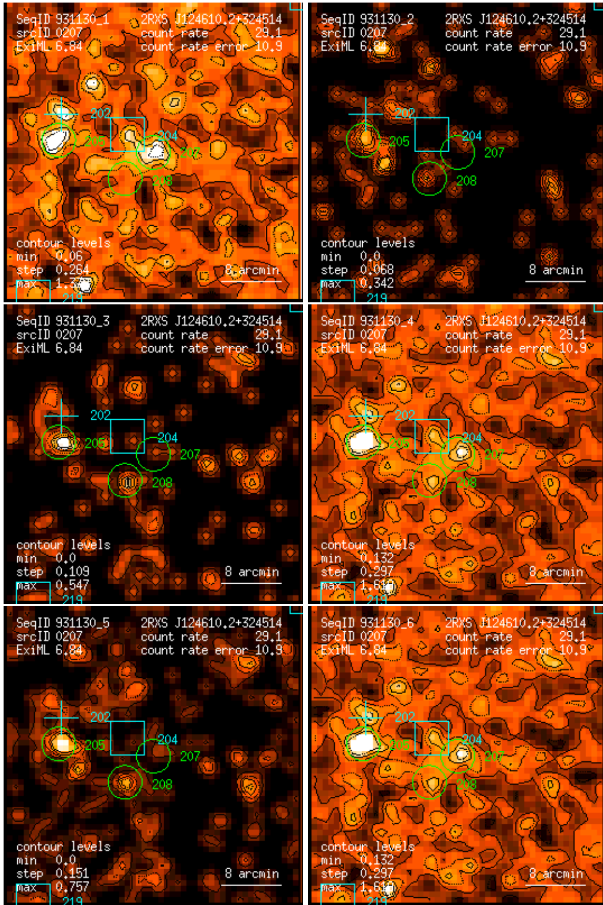
Figure 207: RASS 931130: detection 0207: band rate images, Gaussian filter: (1) PSPC channels 11 – 41, (2) 52 – 90, (3) 91 – 201, (4) 11 – 235, (5) 52 – 201, (6) 11 – 201. Broad band rates in counts/ks. Band rate contour levels in counts/ks/arcmin 2 .
