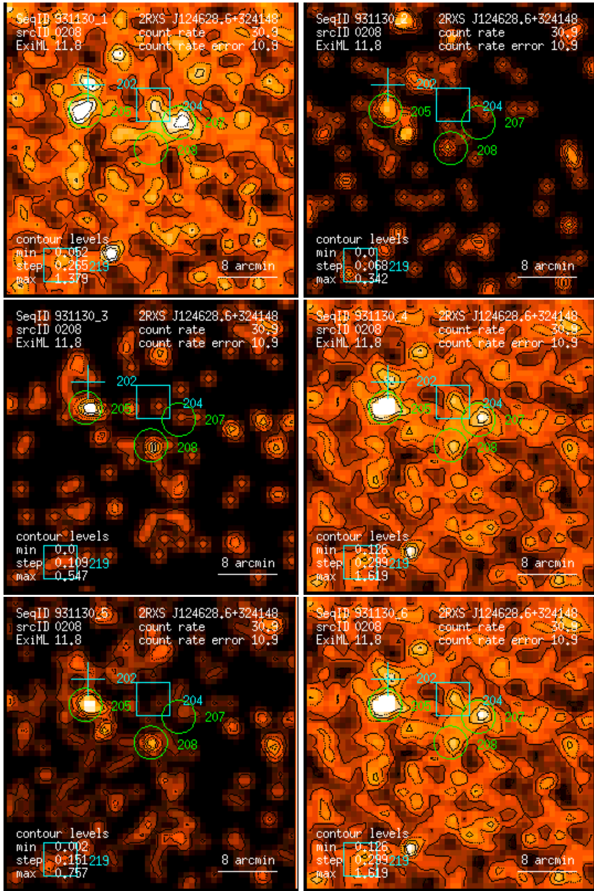
Figure 208: RASS 931130: detection 0208: band rate images, Gaussian filter: (1) PSPC channels 11 – 41, (2) 52 – 90, (3) 91 – 201, (4) 11 – 235, (5) 52 – 201, (6) 11 – 201. Broad band rates in counts/ks. Band rate contour levels in counts/ks/arcmin 2 .
