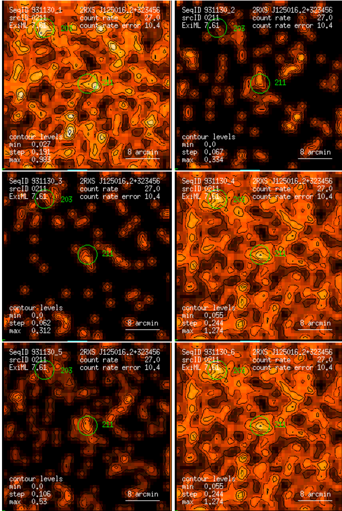
Figure 211: RASS 931130: detection 0211: band rate images, Gaussian filter: (1) PSPC channels 11 – 41, (2) 52 – 90, (3) 91 – 201, (4) 11 – 235, (5) 52 – 201, (6) 11 – 201. Broad band rates in counts/ks. Band rate contour levels in counts/ks/arcmin 2 .
