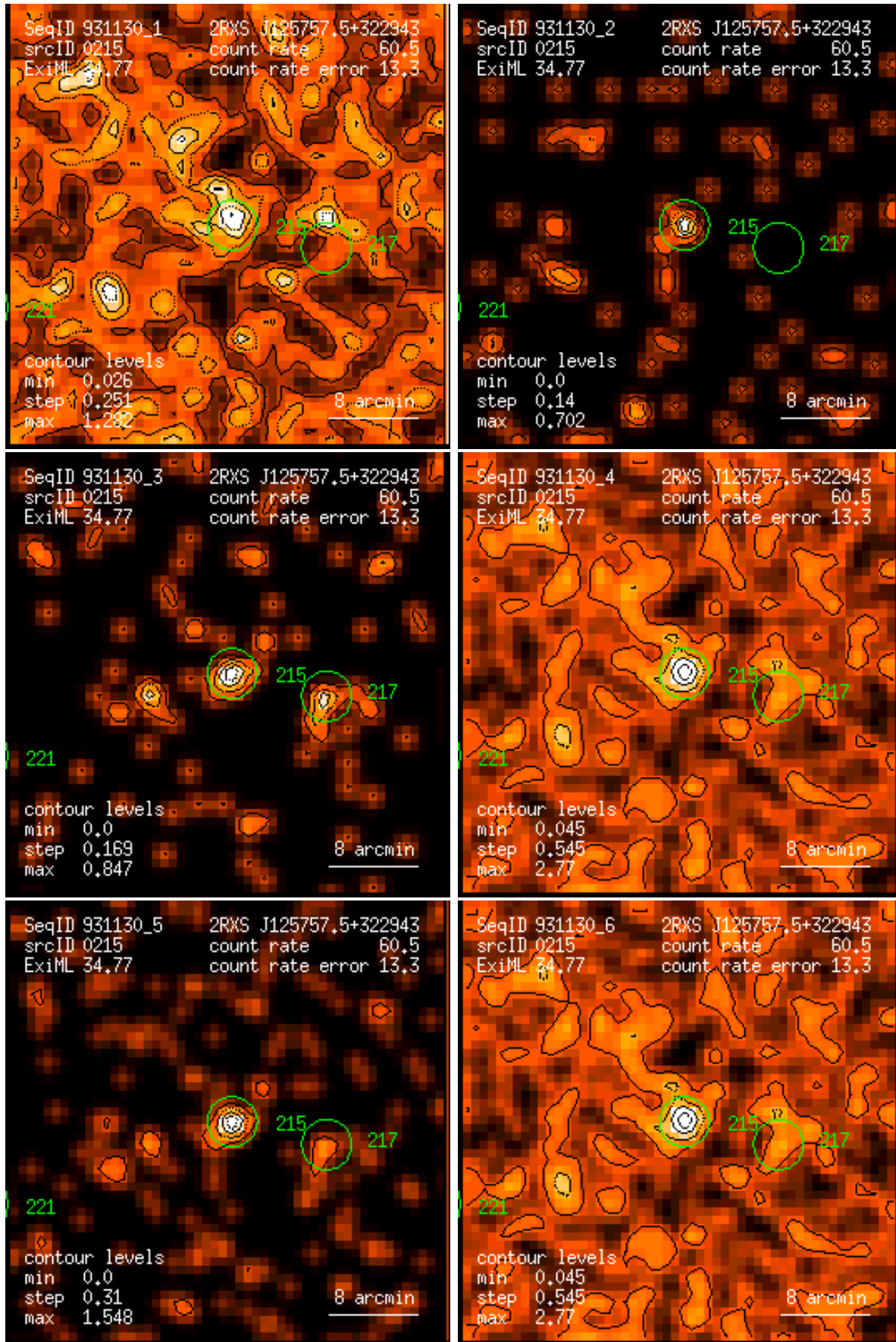
Figure 215: RASS 931130: detection 0215: band rate images, Gaussian filter: (1) PSPC channels 11 – 41, (2) 52 – 90, (3) 91 – 201, (4) 11 – 235, (5) 52 – 201, (6) 11 – 201. Broad band rates in counts/ks. Band rate contour levels in counts/ks/arcmin 2 .
