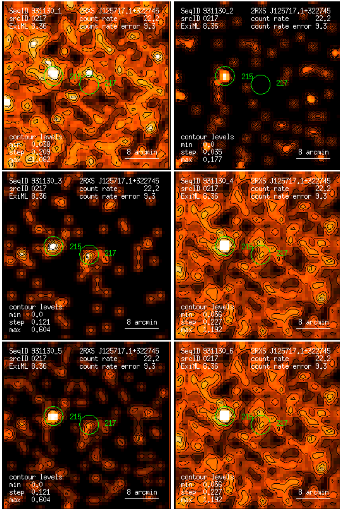
Figure 217: RASS 931130: detection 0217: band rate images, Gaussian filter: (1) PSPC channels 11 – 41, (2) 52 – 90, (3) 91 – 201, (4) 11 – 235, (5) 52 – 201, (6) 11 – 201. Broad band rates in counts/ks. Band rate contour levels in counts/ks/arcmin 2 .
