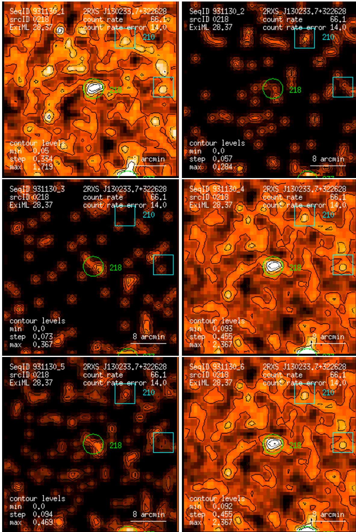
Figure 218: RASS 931130: detection 0218: band rate images, Gaussian filter: (1) PSPC channels 11 – 41, (2) 52 – 90, (3) 91 – 201, (4) 11 – 235, (5) 52 – 201, (6) 11 – 201. Broad band rates in counts/ks. Band rate contour levels in counts/ks/arcmin 2 .
