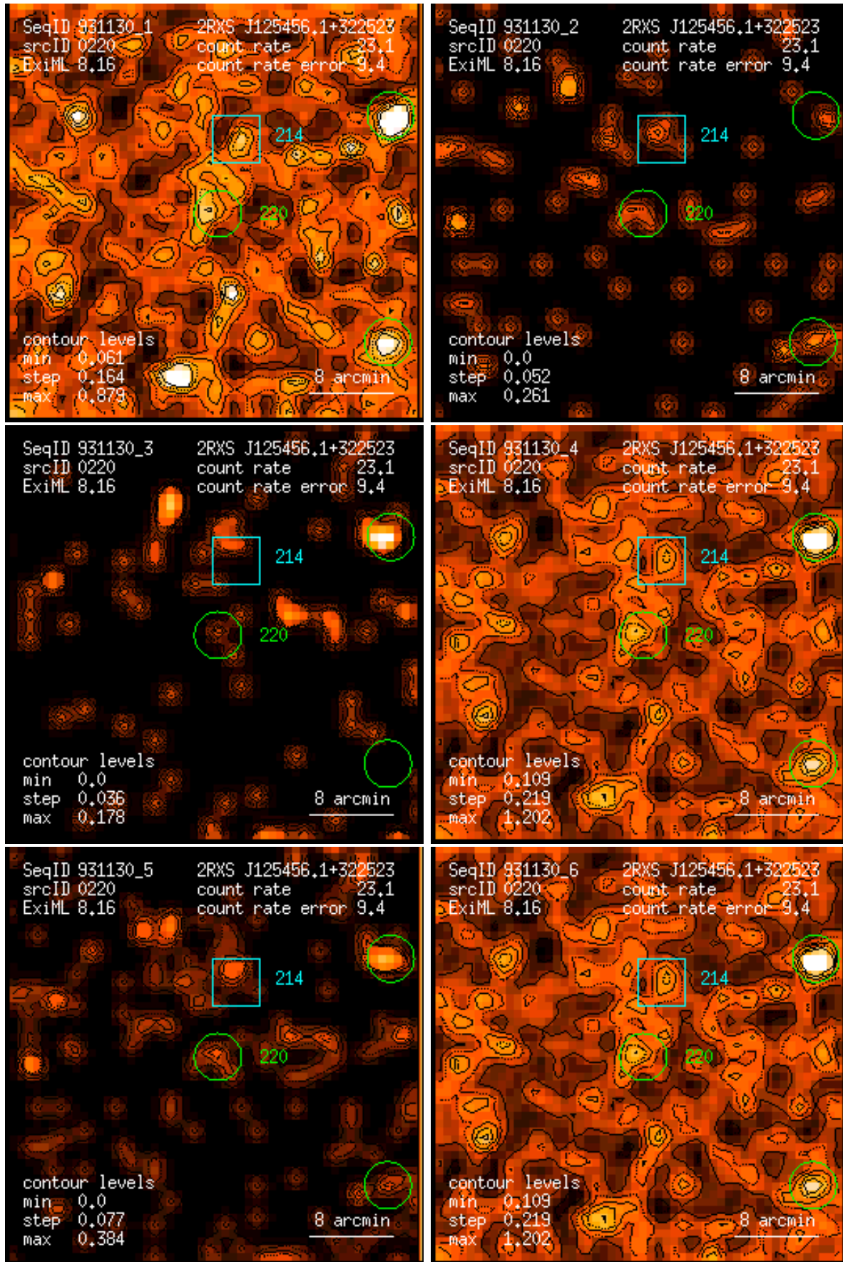
Figure 220: RASS 931130: detection 0220: band rate images, Gaussian filter: (1) PSPC channels 11 – 41, (2) 52 – 90, (3) 91 – 201, (4) 11 – 235, (5) 52 – 201, (6) 11 – 201. Broad band rates in counts/ks. Band rate contour levels in counts/ks/arcmin 2 .
