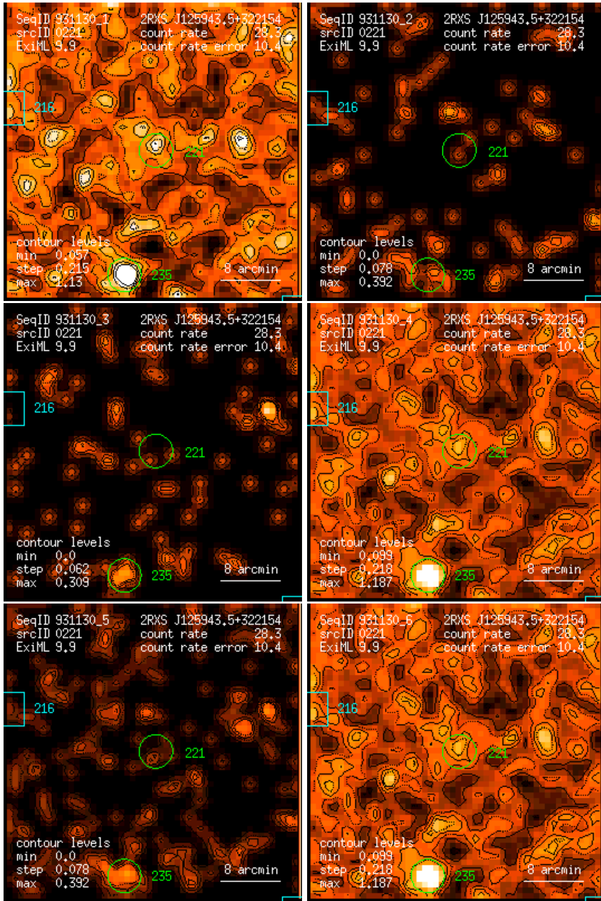
Figure 221: RASS 931130: detection 0221: band rate images, Gaussian filter: (1) PSPC channels 11 – 41, (2) 52 – 90, (3) 91 – 201, (4) 11 – 235, (5) 52 – 201, (6) 11 – 201. Broad band rates in counts/ks. Band rate contour levels in counts/ks/arcmin 2 .
