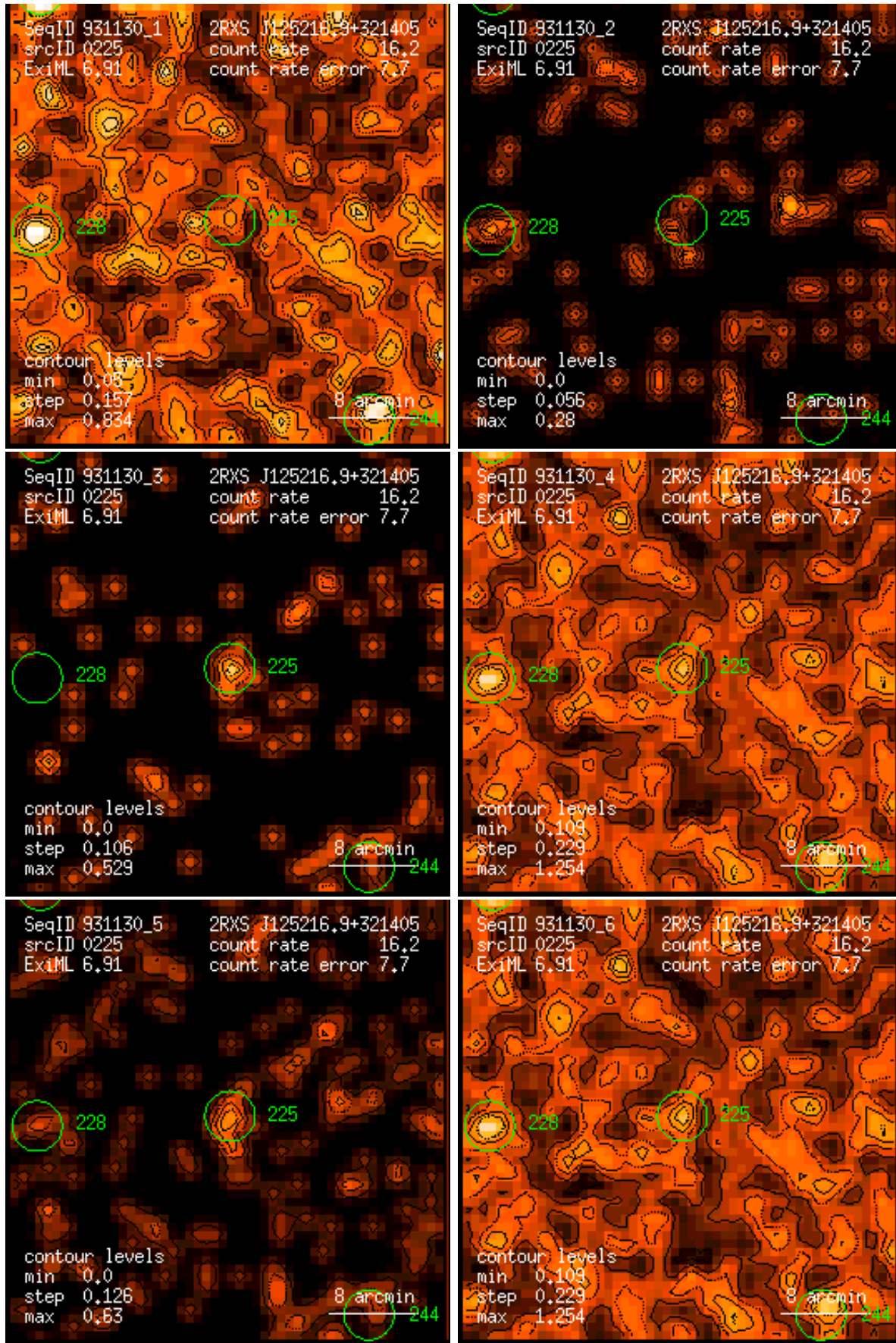
Figure 225: RASS 931130: detection 0225: band rate images, Gaussian filter: (1) PSPC channels 11 – 41, (2) 52 – 90, (3) 91 – 201, (4) 11 – 235, (5) 52 – 201, (6) 11 – 201. Broad band rates in counts/ks. Band rate contour levels in counts/ks/arcmin 2 .
