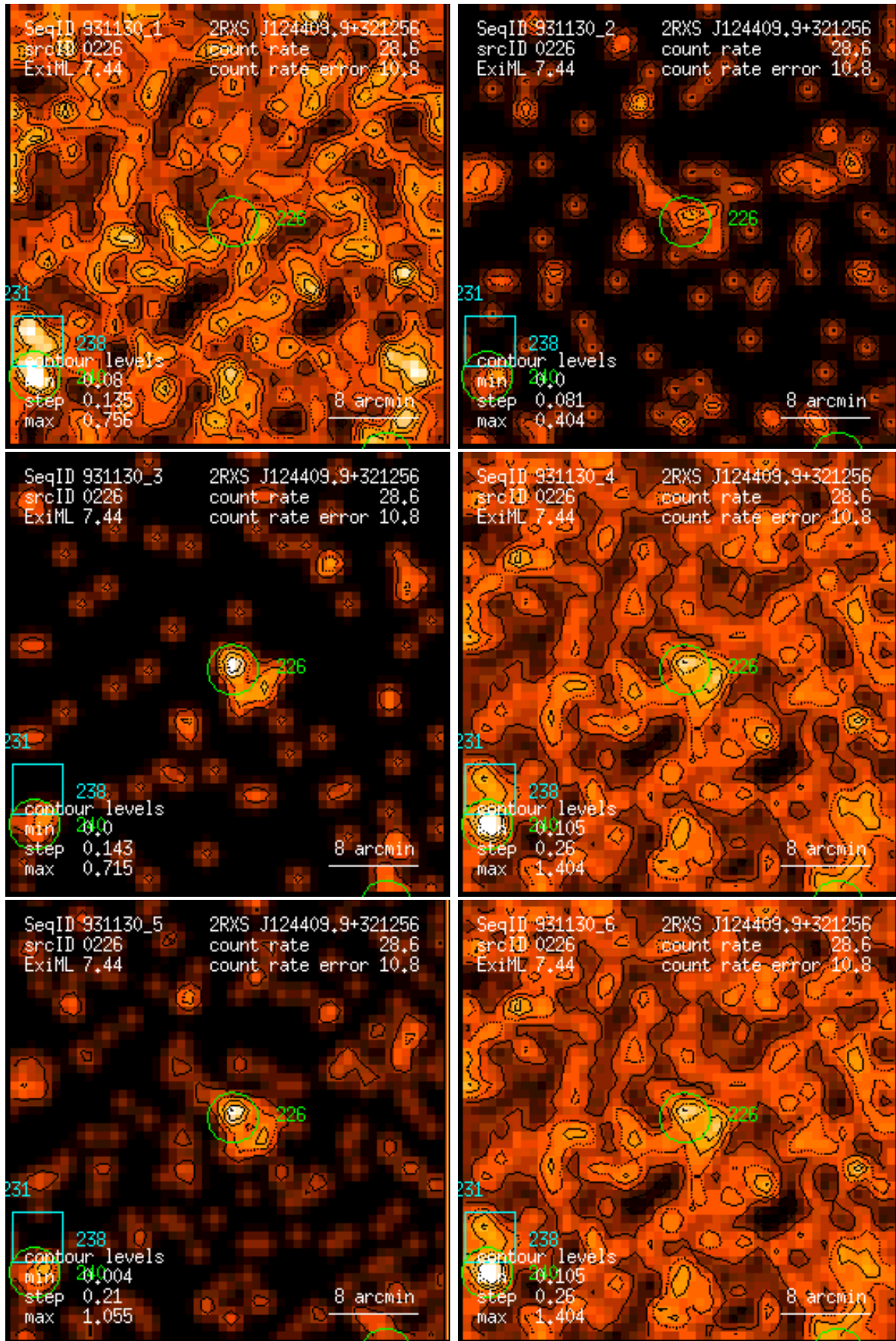
Figure 226: RASS 931130: detection 0226: band rate images, Gaussian filter: (1) PSPC channels 11 – 41, (2) 52 – 90, (3) 91 – 201, (4) 11 – 235, (5) 52 – 201, (6) 11 – 201. Broad band rates in counts/ks. Band rate contour levels in counts/ks/arcmin 2 .
