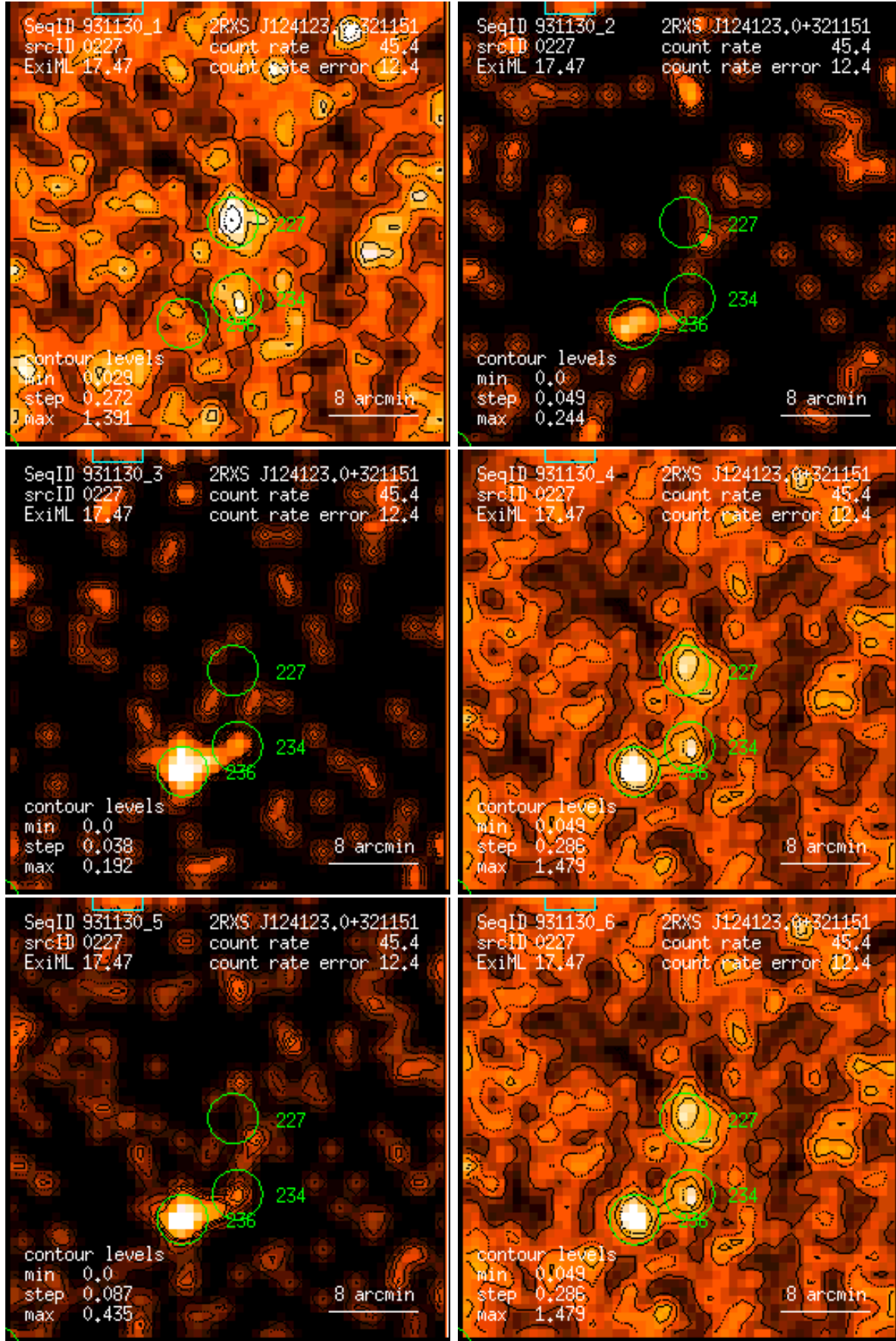
Figure 227: RASS 931130: detection 0227: band rate images, Gaussian filter: (1) PSPC channels 11 – 41, (2) 52 – 90, (3) 91 – 201, (4) 11 – 235, (5) 52 – 201, (6) 11 – 201. Broad band rates in counts/ks. Band rate contour levels in counts/ks/arcmin 2 .
