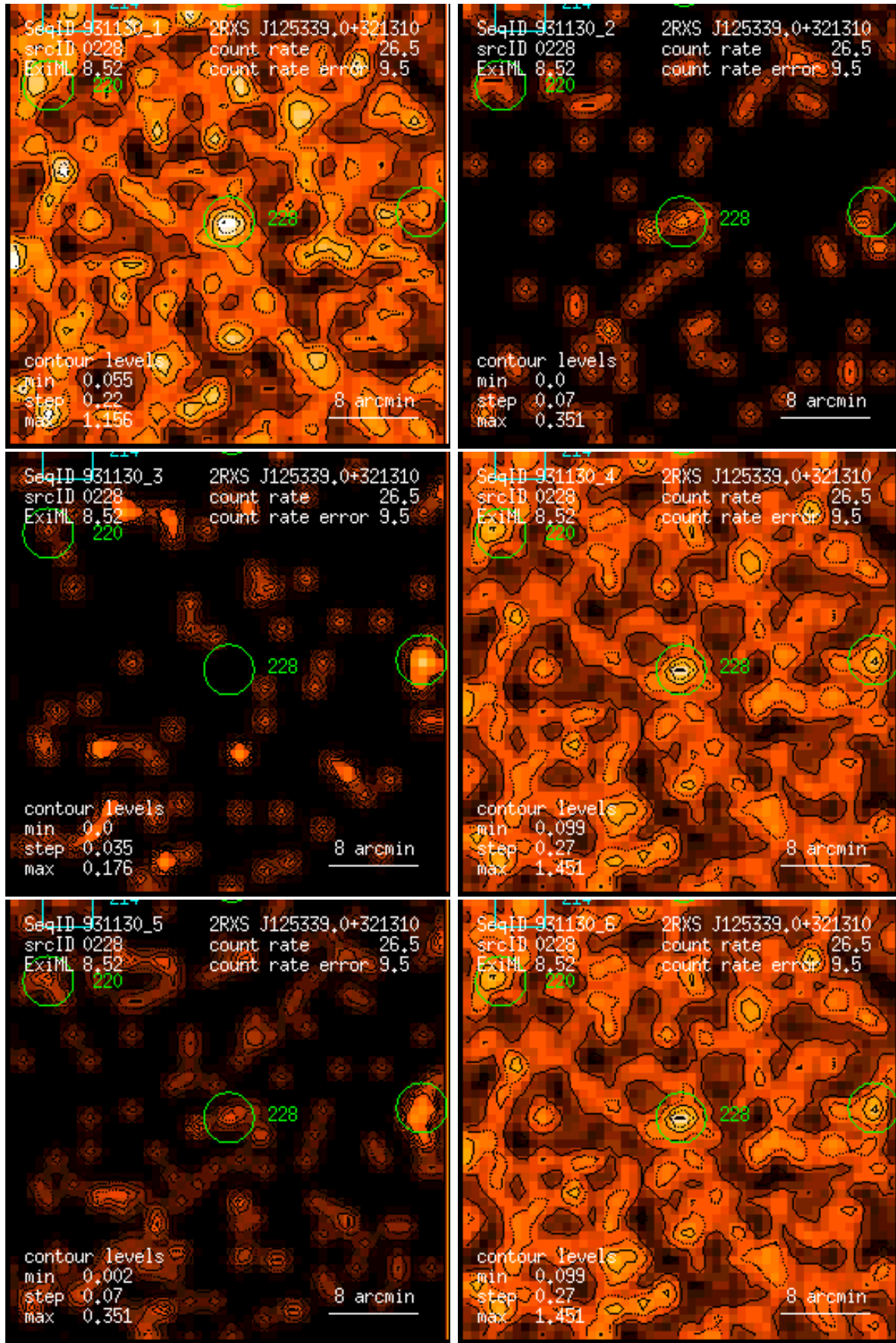
Figure 228: RASS 931130: detection 0228: band rate images, Gaussian filter: (1) PSPC channels 11 – 41, (2) 52 – 90, (3) 91 – 201, (4) 11 – 235, (5) 52 – 201, (6) 11 – 201. Broad band rates in counts/ks. Band rate contour levels in counts/ks/arcmin 2 .
