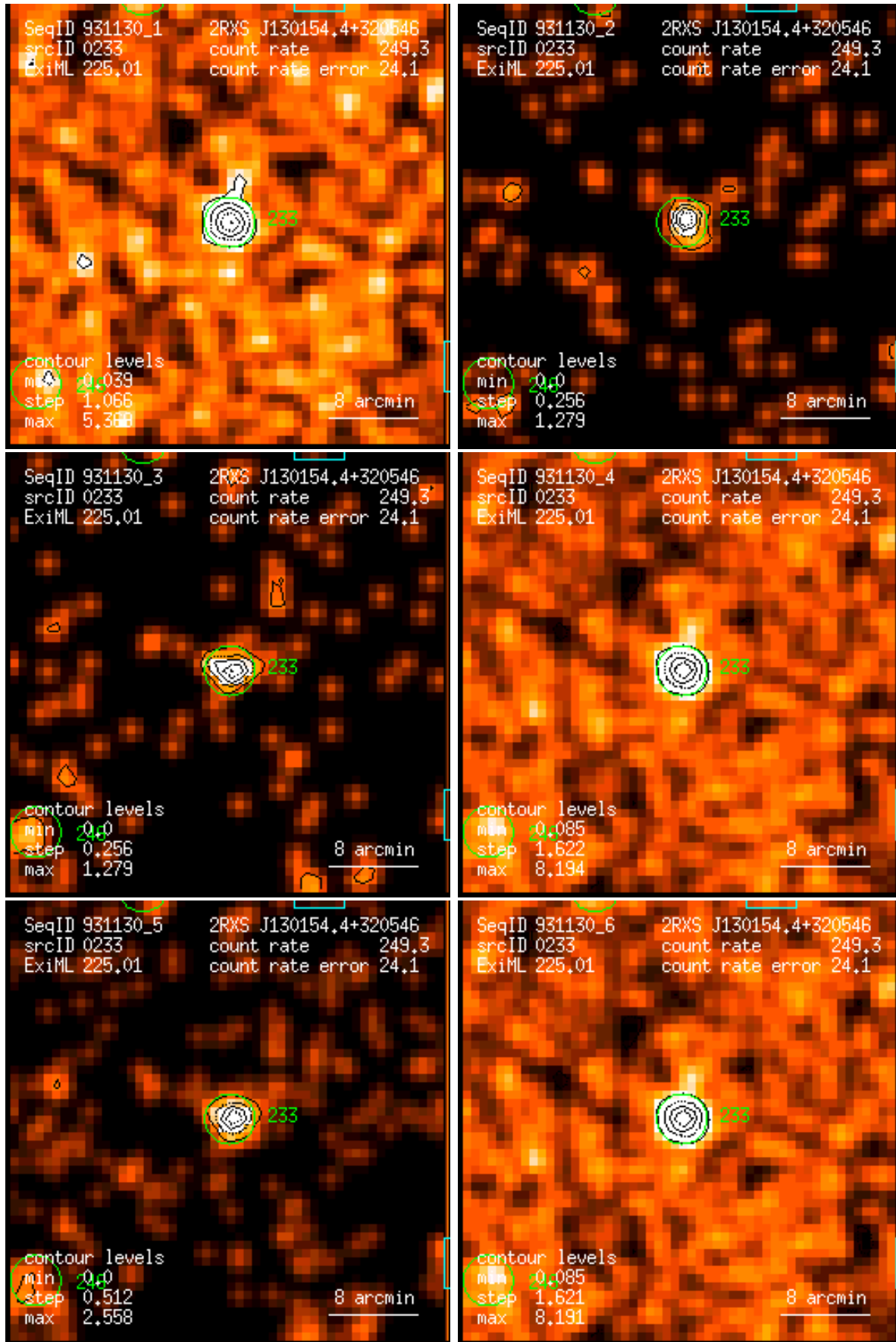
Figure 233: RASS 931130: detection 0233: band rate images, Gaussian filter: (1) PSPC channels 11 – 41, (2) 52 – 90, (3) 91 – 201, (4) 11 – 235, (5) 52 – 201, (6) 11 – 201. Broad band rates in counts/ks. Band rate contour levels in counts/ks/arcmin 2 .
