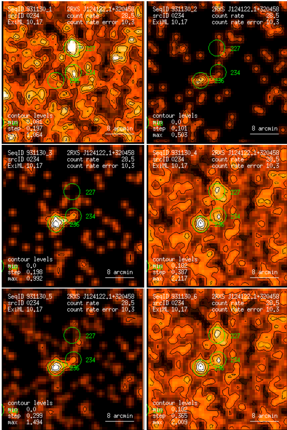
Figure 234: RASS 931130: detection 0234: band rate images, Gaussian filter: (1) PSPC channels 11 – 41, (2) 52 – 90, (3) 91 – 201, (4) 11 – 235, (5) 52 – 201, (6) 11 – 201. Broad band rates in counts/ks. Band rate contour levels in counts/ks/arcmin 2 .
