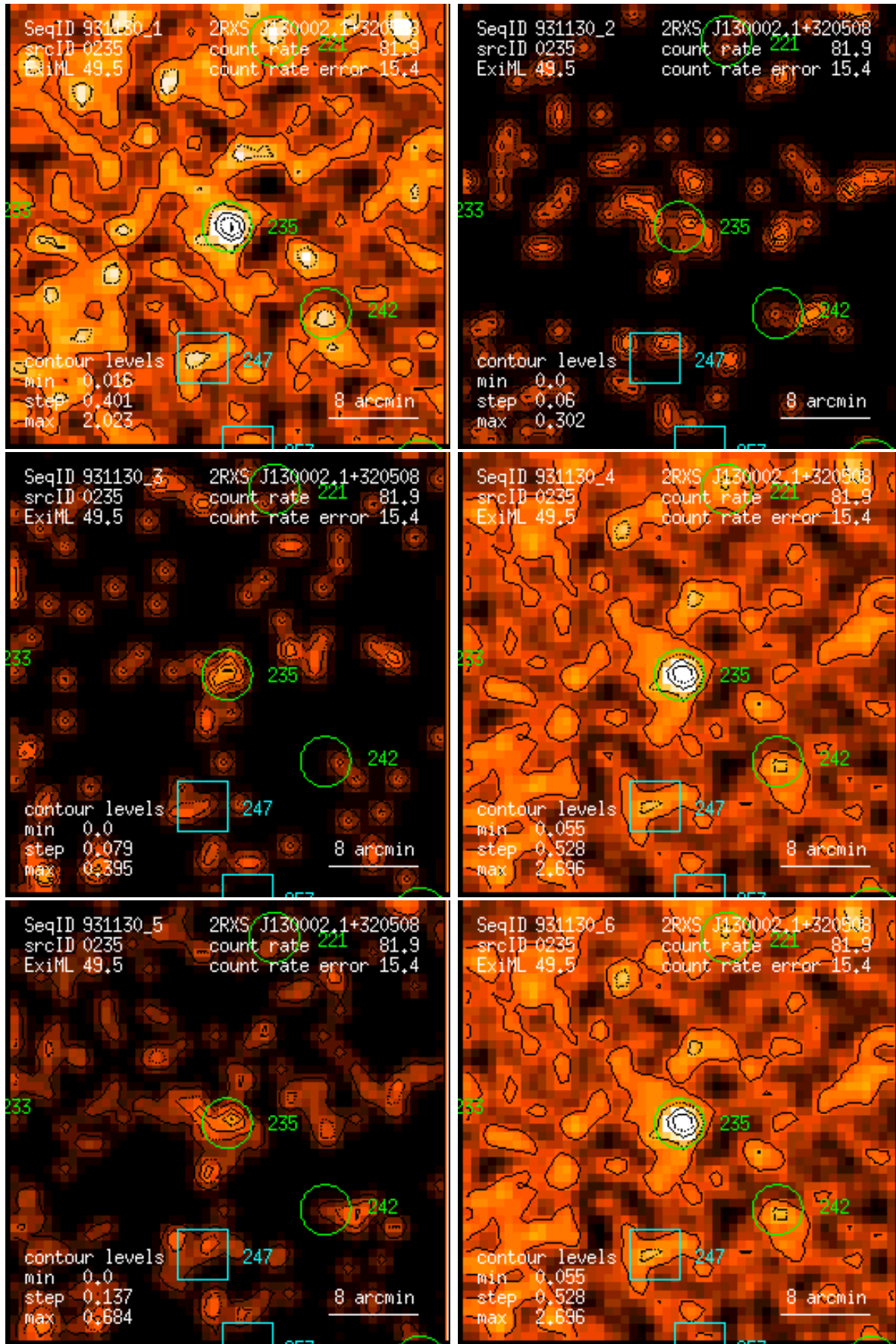
Figure 235: RASS 931130: detection 0235: band rate images, Gaussian filter: (1) PSPC channels 11 – 41, (2) 52 – 90, (3) 91 – 201, (4) 11 – 235, (5) 52 – 201, (6) 11 – 201. Broad band rates in counts/ks. Band rate contour levels in counts/ks/arcmin 2 .
