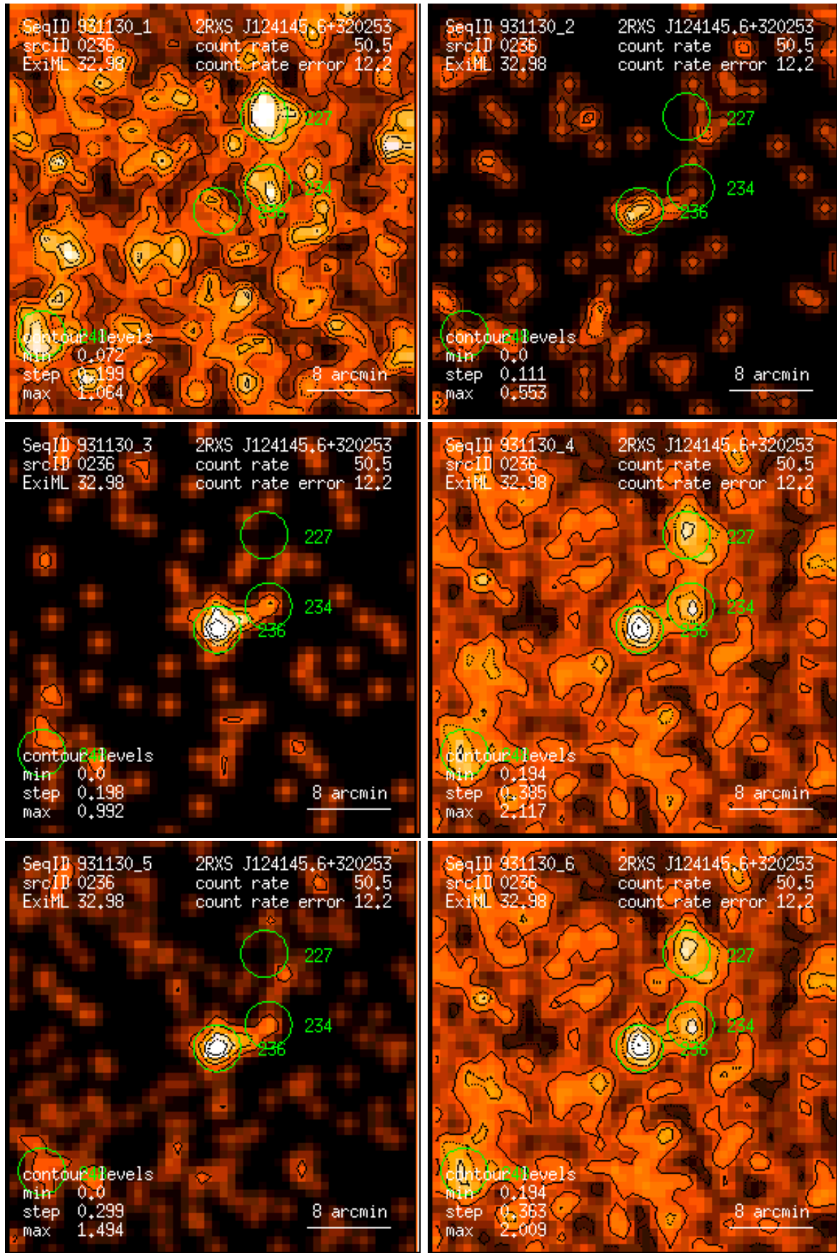
Figure 236: RASS 931130: detection 0236: band rate images, Gaussian filter: (1) PSPC channels 11 – 41, (2) 52 – 90, (3) 91 – 201, (4) 11 – 235, (5) 52 – 201, (6) 11 – 201. Broad band rates in counts/ks. Band rate contour levels in counts/ks/arcmin 2 .
