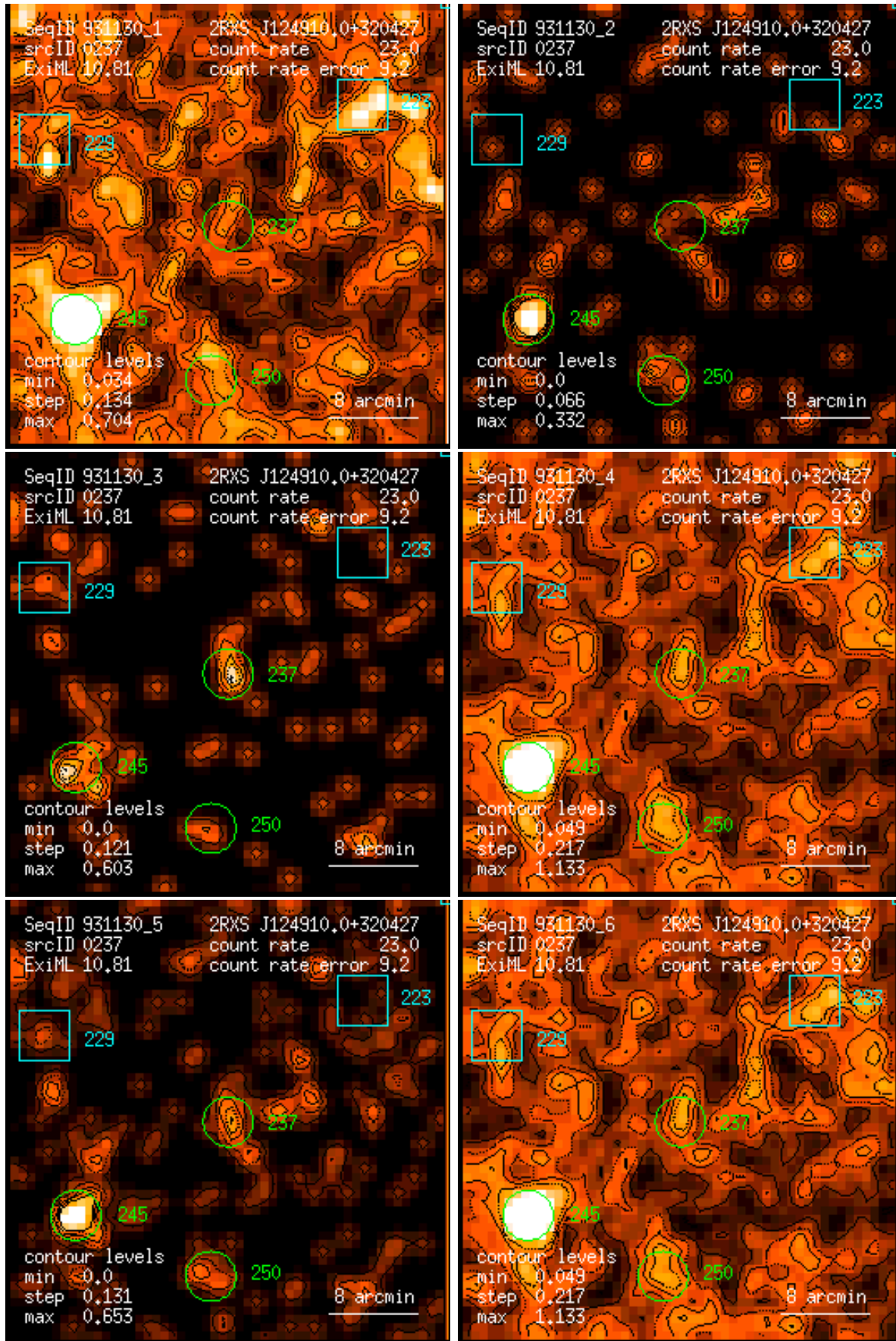
Figure 237: RASS 931130: detection 0237: band rate images, Gaussian filter: (1) PSPC channels 11 – 41, (2) 52 – 90, (3) 91 – 201, (4) 11 – 235, (5) 52 – 201, (6) 11 – 201. Broad band rates in counts/ks. Band rate contour levels in counts/ks/arcmin 2 .
