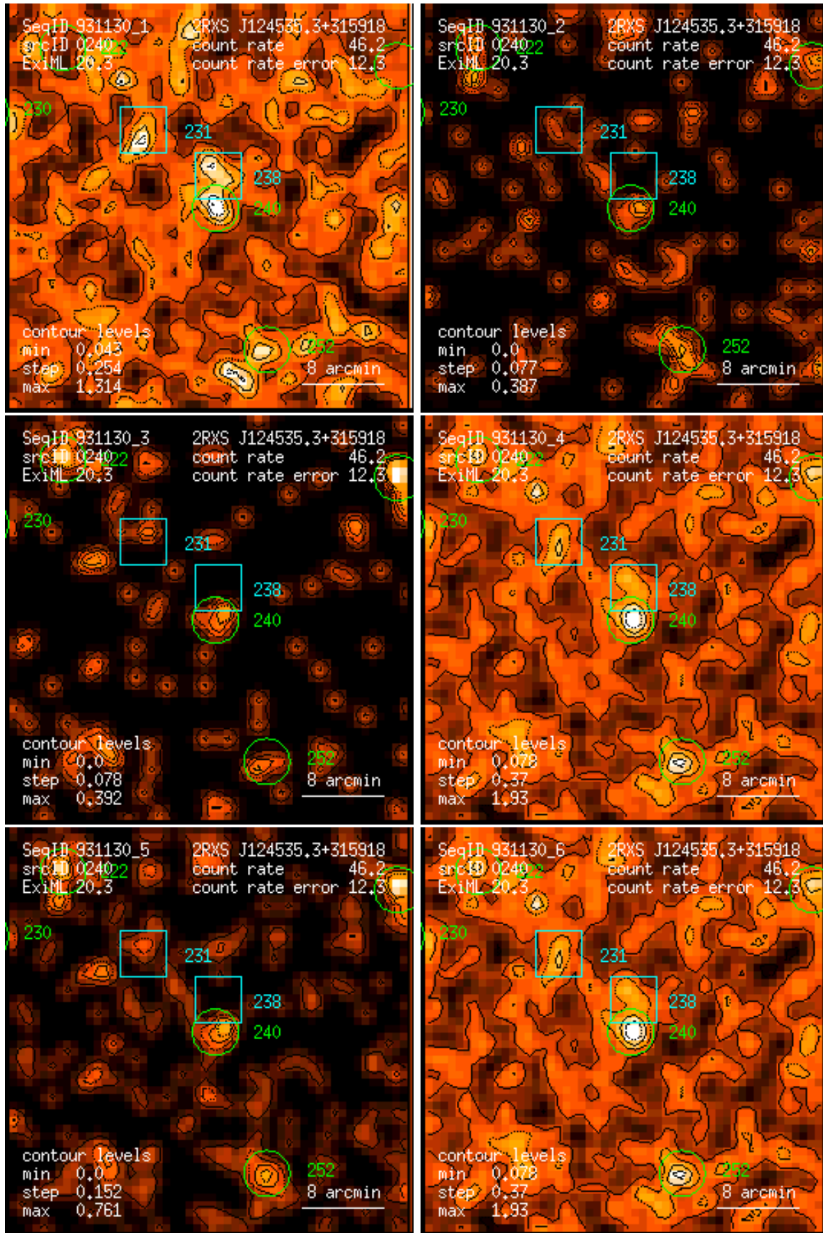
Figure 240: RASS 931130: detection 0240: band rate images, Gaussian filter: (1) PSPC channels 11 – 41, (2) 52 – 90, (3) 91 – 201, (4) 11 – 235, (5) 52 – 201, (6) 11 – 201. Broad band rates in counts/ks. Band rate contour levels in counts/ks/arcmin 2 .
