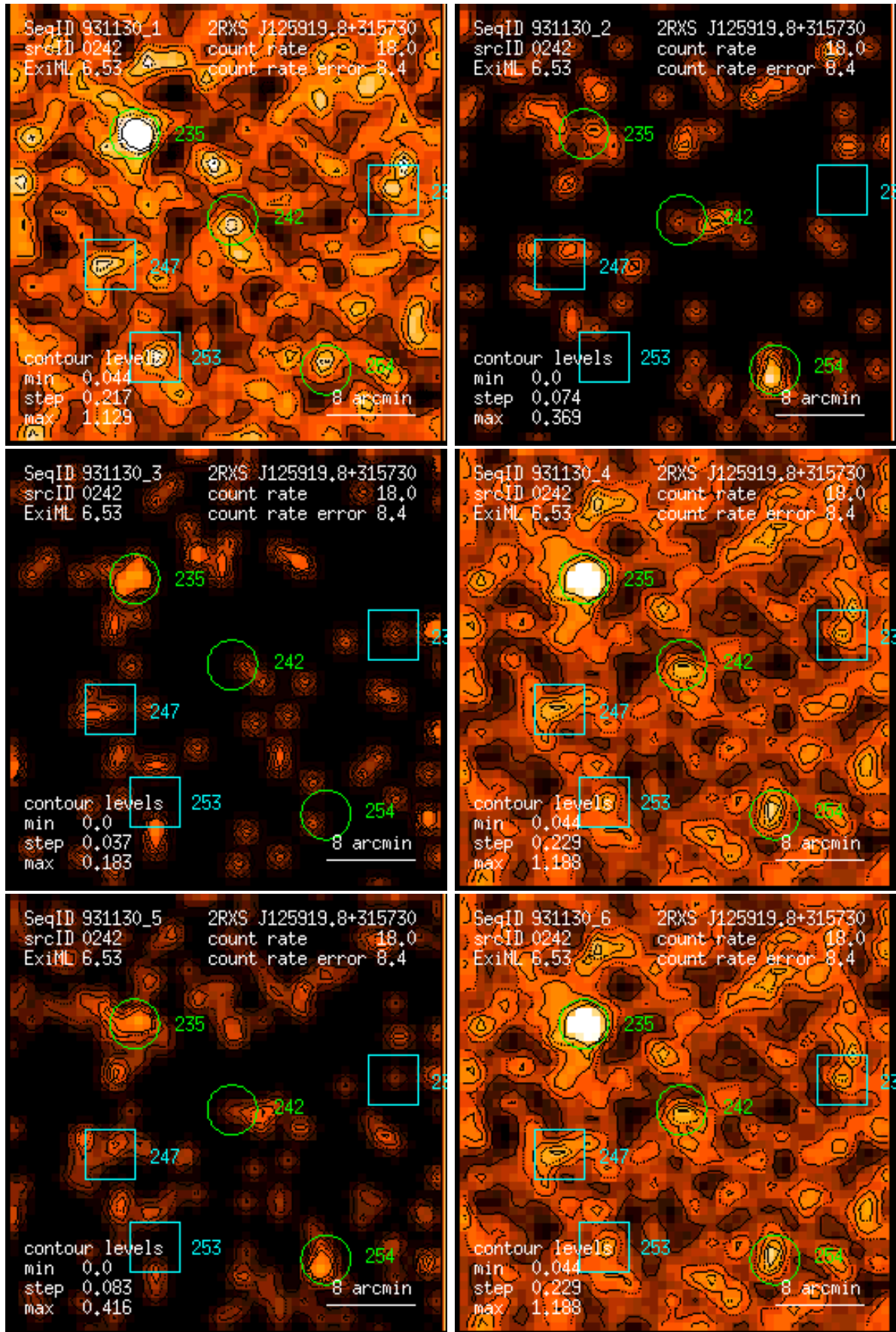
Figure 242: RASS 931130: detection 0242: band rate images, Gaussian filter: (1) PSPC channels 11 – 41, (2) 52 – 90, (3) 91 – 201, (4) 11 – 235, (5) 52 – 201, (6) 11 – 201. Broad band rates in counts/ks. Band rate contour levels in counts/ks/arcmin 2 .
