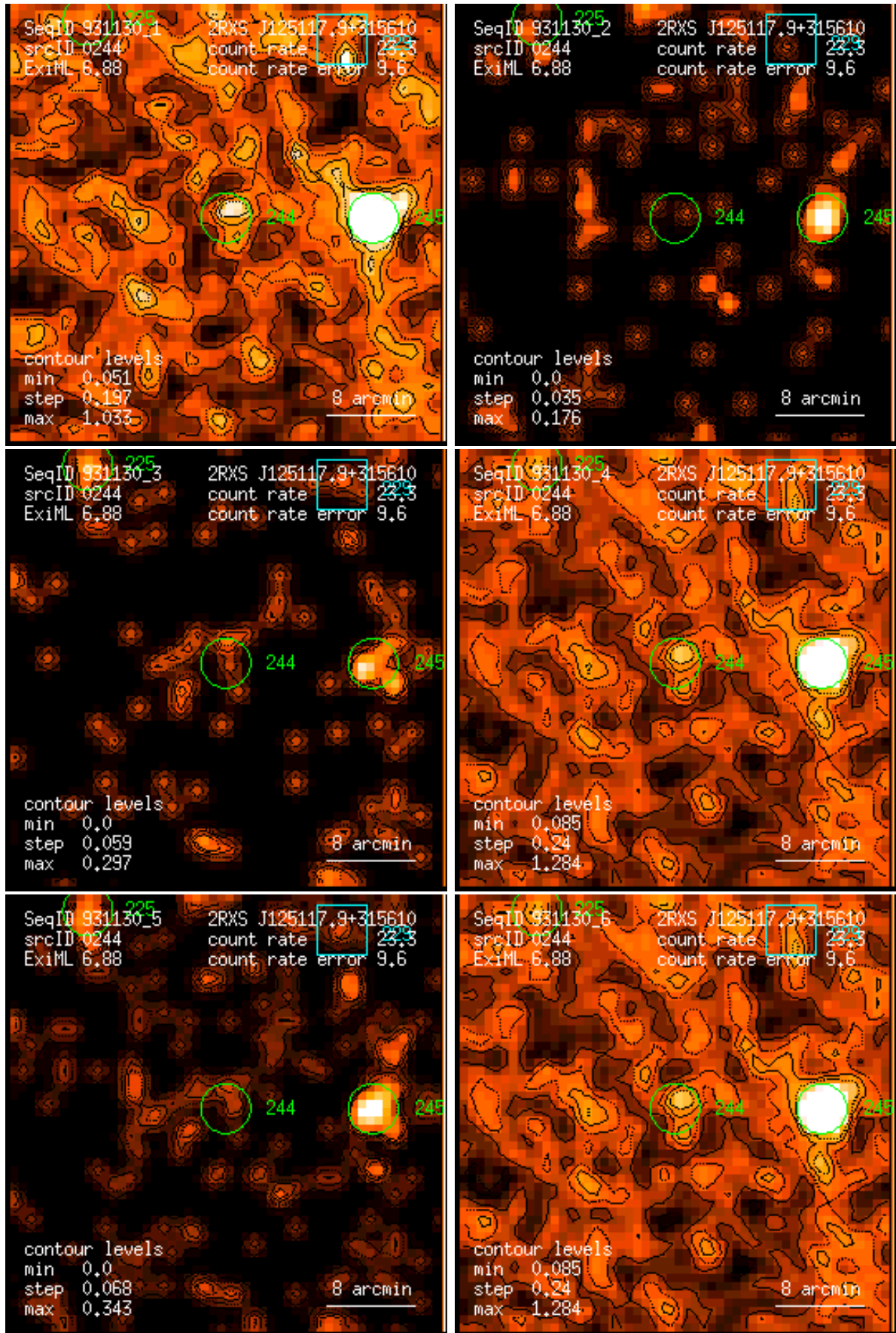
Figure 244: RASS 931130: detection 0244: band rate images, Gaussian filter: (1) PSPC channels 11 – 41, (2) 52 – 90, (3) 91 – 201, (4) 11 – 235, (5) 52 – 201, (6) 11 – 201. Broad band rates in counts/ks. Band rate contour levels in counts/ks/arcmin 2 .
