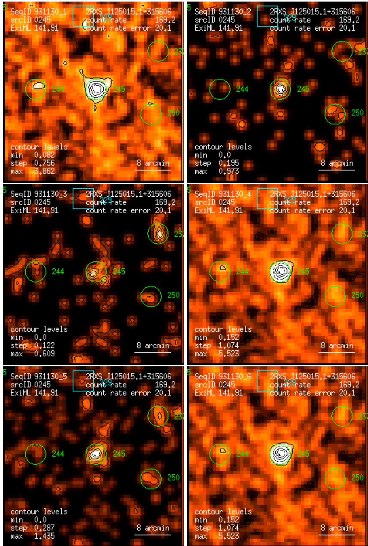
Figure 245: RASS 931130: detection 0245: band rate images, Gaussian filter: (1) PSPC channels 11 – 41, (2) 52 – 90, (3) 91 – 201, (4) 11 – 235, (5) 52 – 201, (6) 11 – 201. Broad band rates in counts/ks. Band rate contour levels in counts/ks/arcmin 2 .
