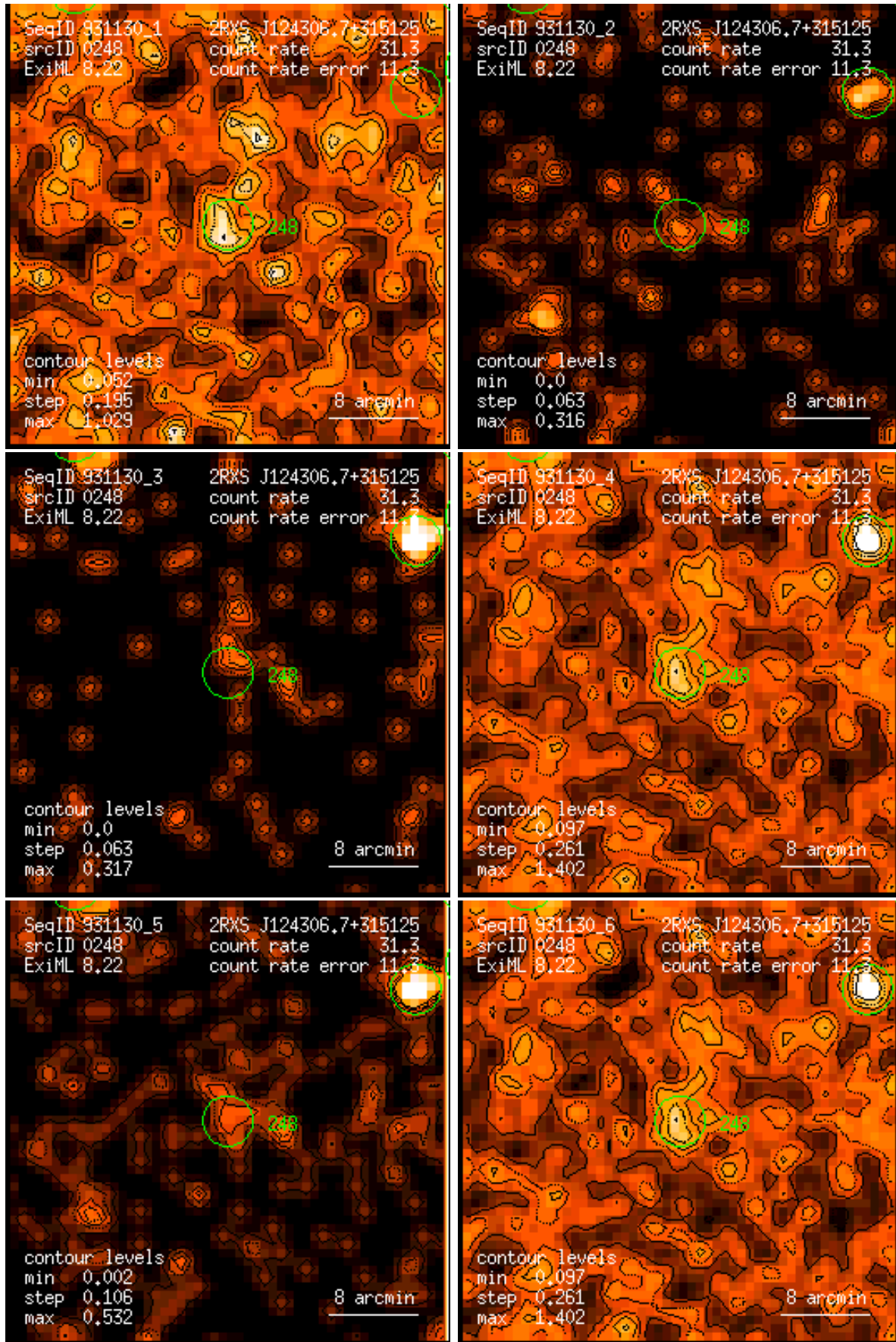
Figure 248: RASS 931130: detection 0248: band rate images, Gaussian filter: (1) PSPC channels 11 – 41, (2) 52 – 90, (3) 91 – 201, (4) 11 – 235, (5) 52 – 201, (6) 11 – 201. Broad band rates in counts/ks. Band rate contour levels in counts/ks/arcmin 2 .
