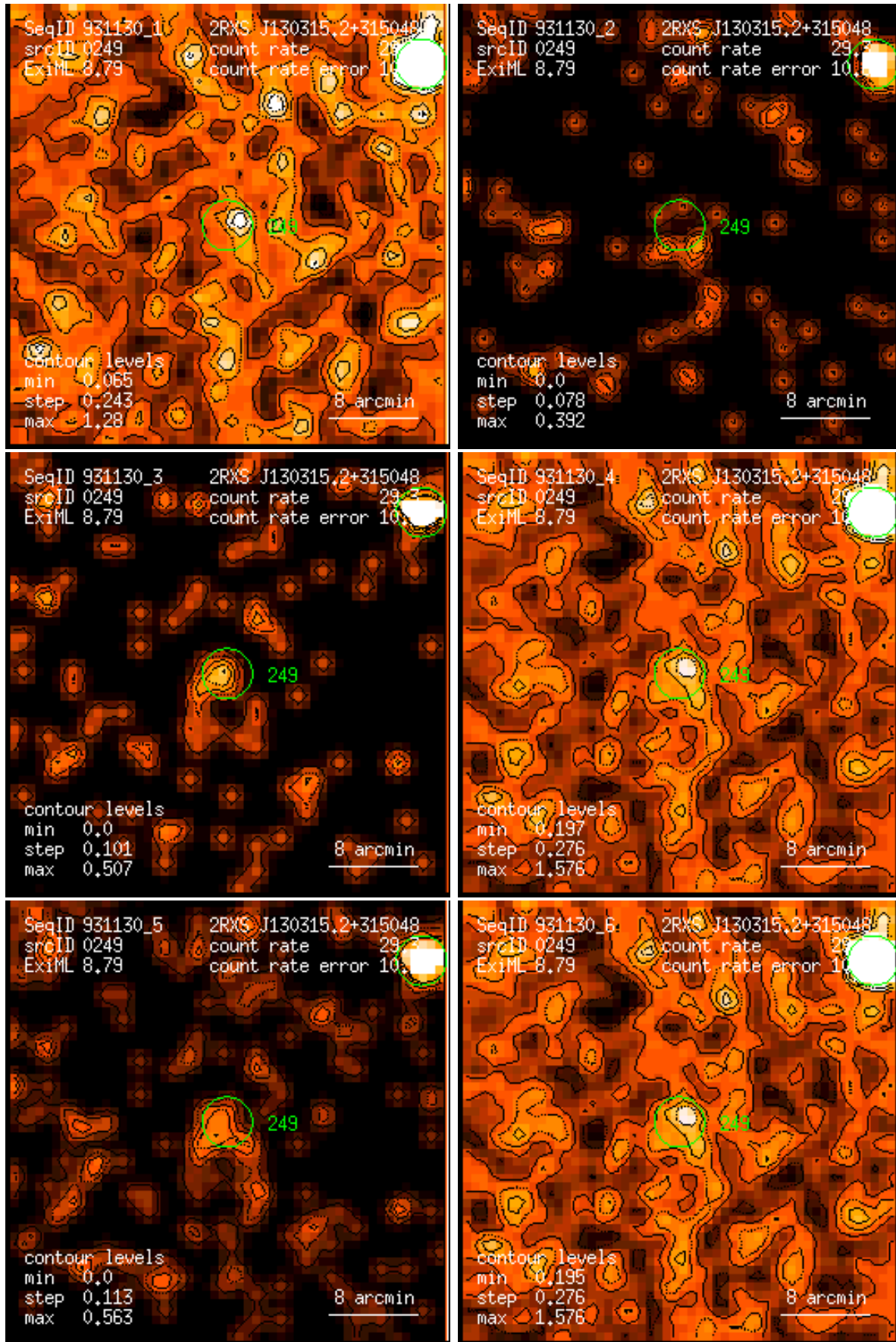
Figure 249: RASS 931130: detection 0249: band rate images, Gaussian filter: (1) PSPC channels 11 – 41, (2) 52 – 90, (3) 91 – 201, (4) 11 – 235, (5) 52 – 201, (6) 11 – 201. Broad band rates in counts/ks. Band rate contour levels in counts/ks/arcmin 2 .
