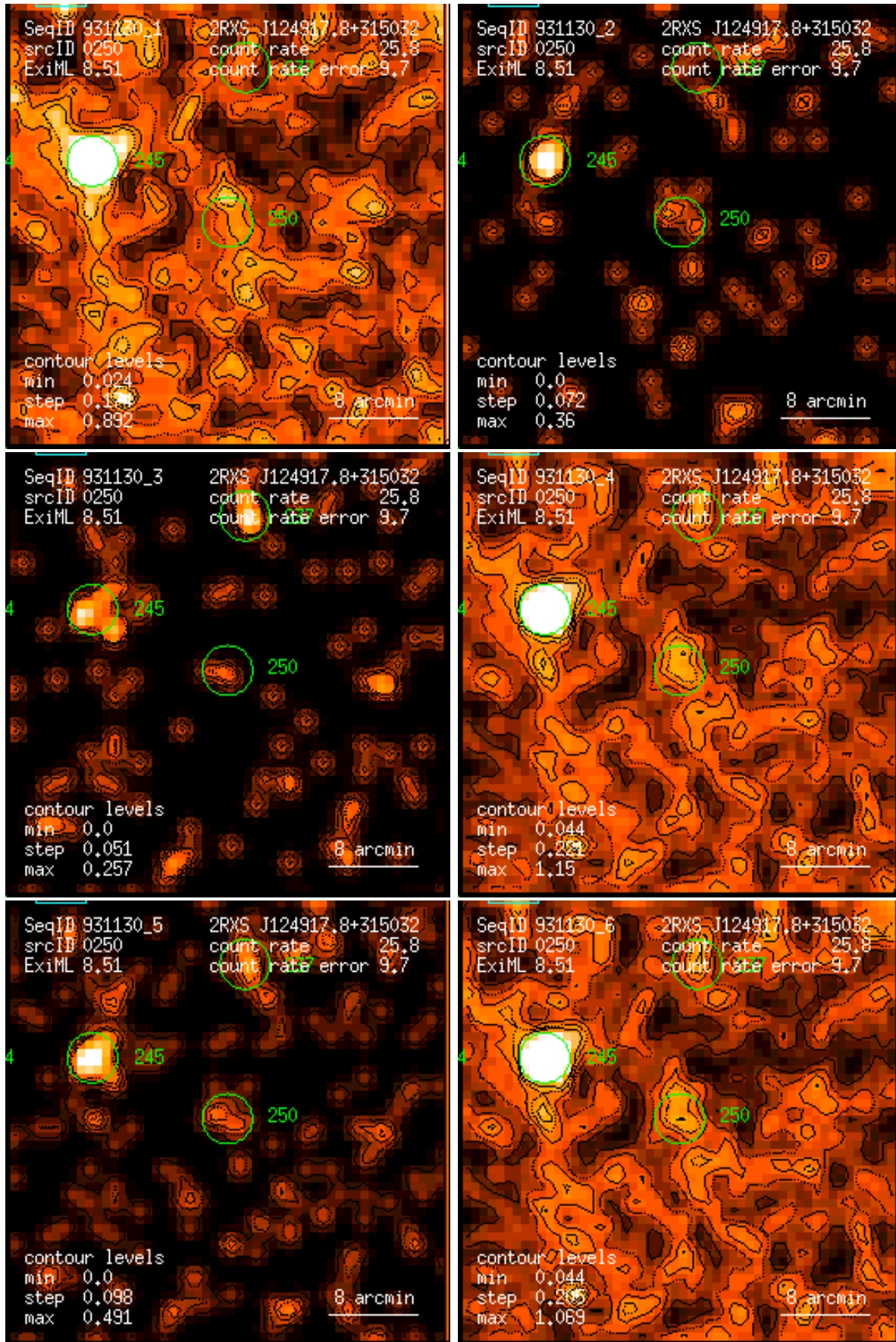
Figure 250: RASS 931130: detection 0250: band rate images, Gaussian filter: (1) PSPC channels 11 – 41, (2) 52 – 90, (3) 91 – 201, (4) 11 – 235, (5) 52 – 201, (6) 11 – 201. Broad band rates in counts/ks. Band rate contour levels in counts/ks/arcmin 2 .
