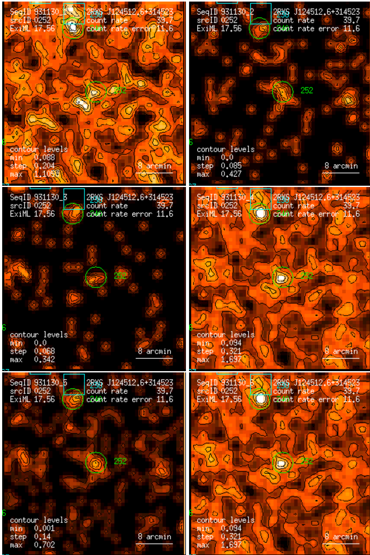
Figure 252: RASS 931130: detection 0252: band rate images, Gaussian filter: (1) PSPC channels 11 – 41, (2) 52 – 90, (3) 91 – 201, (4) 11 – 235, (5) 52 – 201, (6) 11 – 201. Broad band rates in counts/ks. Band rate contour levels in counts/ks/arcmin 2 .
