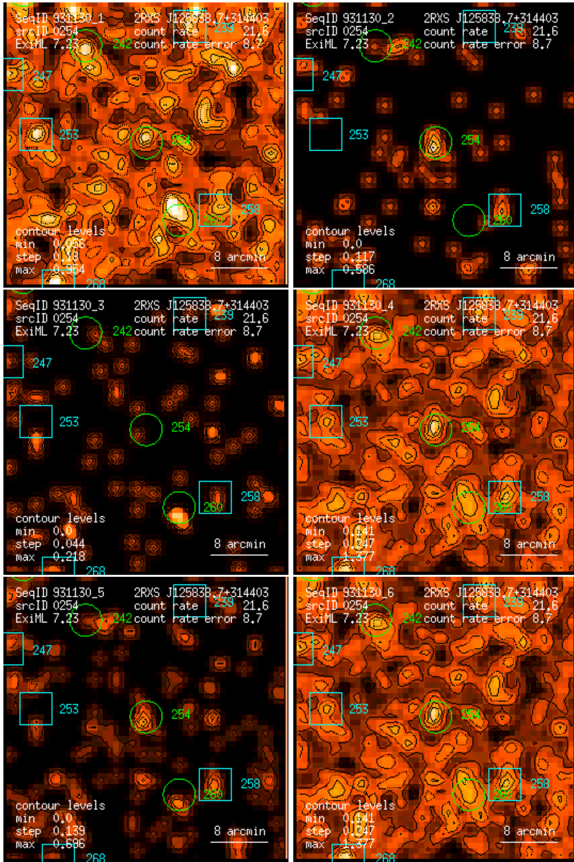
Figure 254: RASS 931130: detection 0254: band rate images, Gaussian filter: (1) PSPC channels 11 – 41, (2) 52 – 90, (3) 91 – 201, (4) 11 – 235, (5) 52 – 201, (6) 11 – 201. Broad band rates in counts/ks. Band rate contour levels in counts/ks/arcmin 2 .
