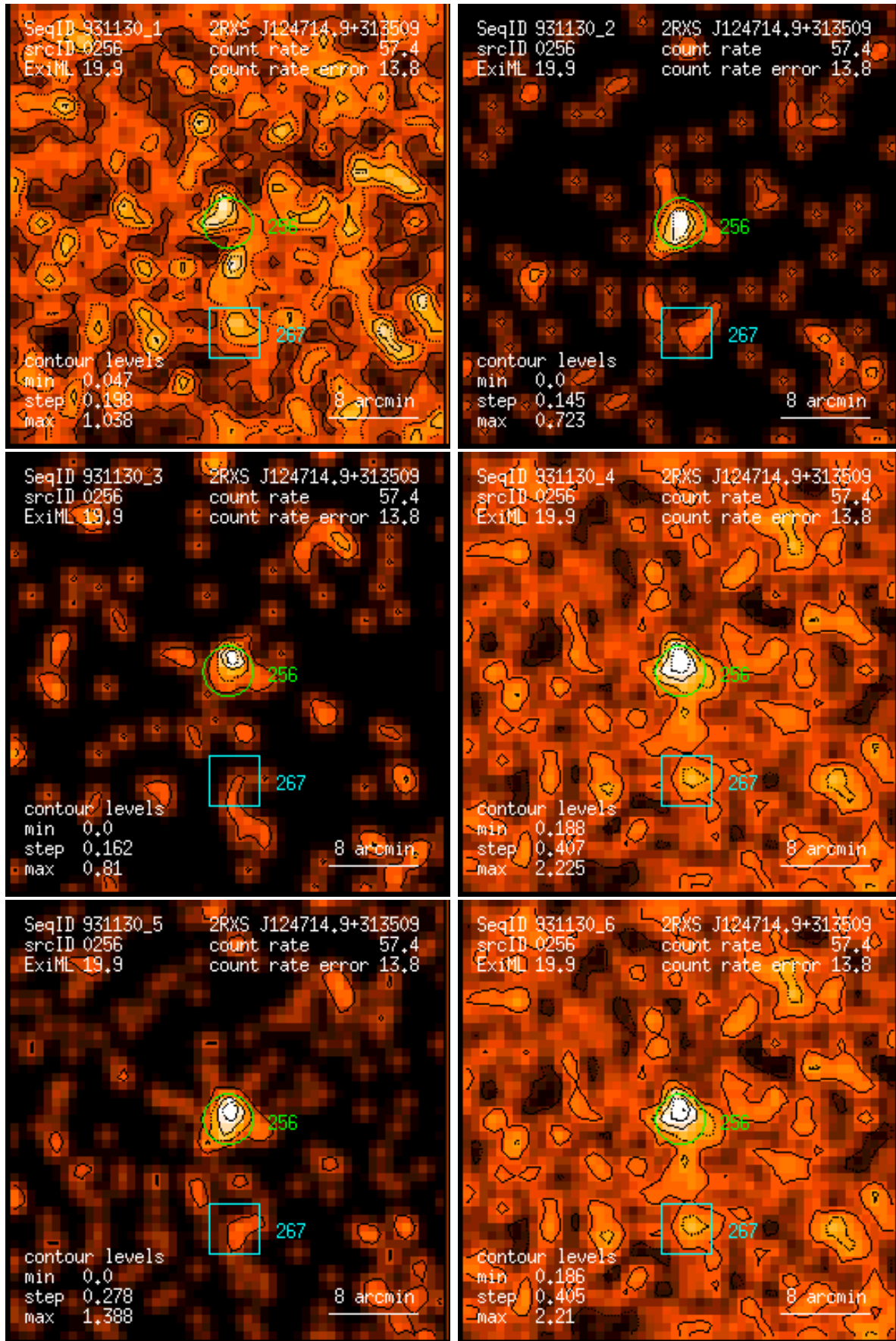
Figure 256: RASS 931130: detection 0256: band rate images, Gaussian filter: (1) PSPC channels 11 – 41, (2) 52 – 90, (3) 91 – 201, (4) 11 – 235, (5) 52 – 201, (6) 11 – 201. Broad band rates in counts/ks. Band rate contour levels in counts/ks/arcmin 2 .
