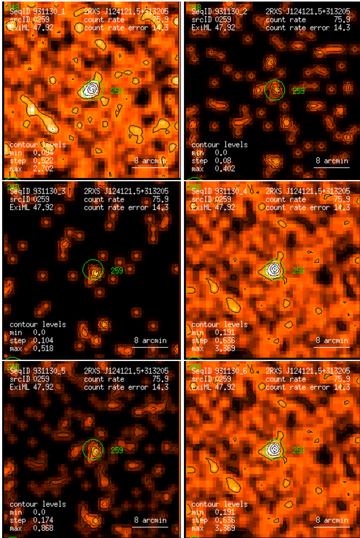
Figure 259: RASS 931130: detection 0259: band rate images, Gaussian filter: (1) PSPC channels 11 – 41, (2) 52 – 90, (3) 91 – 201, (4) 11 – 235, (5) 52 – 201, (6) 11 – 201. Broad band rates in counts/ks. Band rate contour levels in counts/ks/arcmin 2 .
