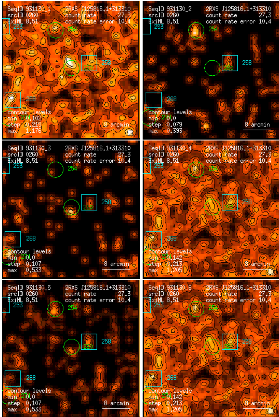
Figure 260: RASS 931130: detection 0260: band rate images, Gaussian filter: (1) PSPC channels 11 – 41, (2) 52 – 90, (3) 91 – 201, (4) 11 – 235, (5) 52 – 201, (6) 11 – 201. Broad band rates in counts/ks. Band rate contour levels in counts/ks/arcmin 2 .
