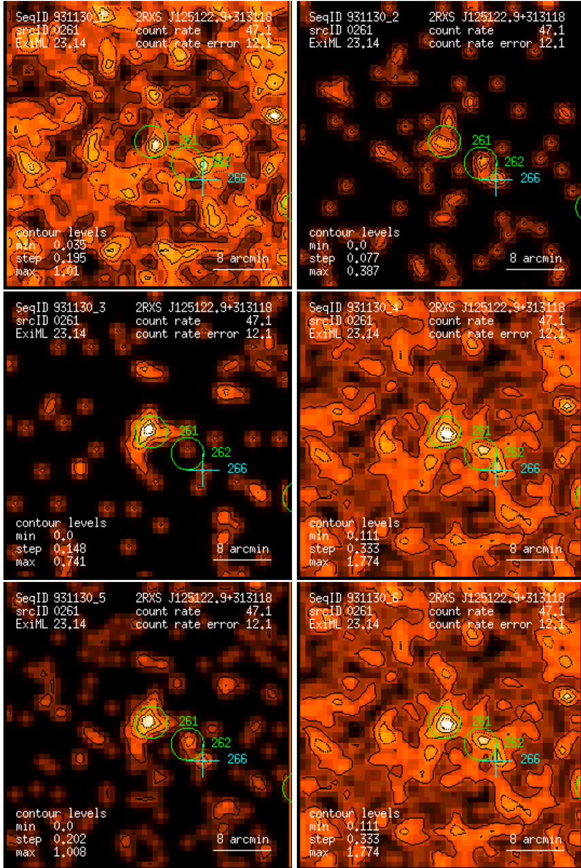
Figure 261: RASS 931130: detection 0261: band rate images, Gaussian filter: (1) PSPC channels 11 – 41, (2) 52 – 90, (3) 91 – 201, (4) 11 – 235, (5) 52 – 201, (6) 11 – 201. Broad band rates in counts/ks. Band rate contour levels in counts/ks/arcmin 2 .
