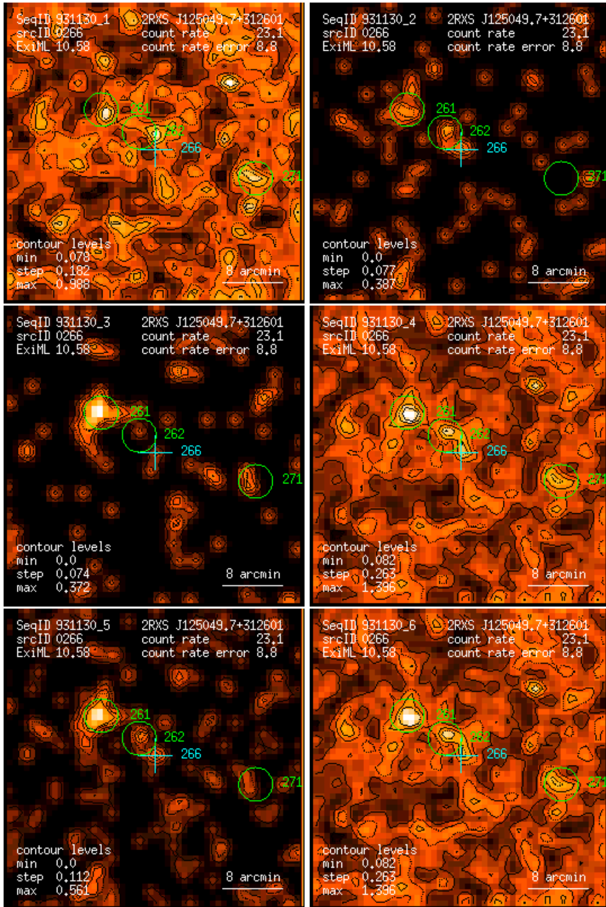
Figure 266: RASS 931130: detection 0266: band rate images, Gaussian filter: (1) PSPC channels 11 – 41, (2) 52 – 90, (3) 91 – 201, (4) 11 – 235, (5) 52 – 201, (6) 11 – 201. Broad band rates in counts/ks. Band rate contour levels in counts/ks/arcmin 2 .
