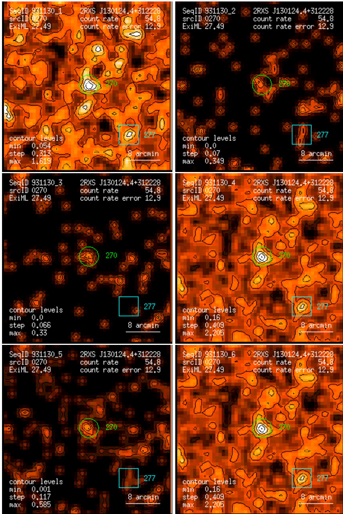
Figure 270: RASS 931130: detection 0270: band rate images, Gaussian filter: (1) PSPC channels 11 – 41, (2) 52 – 90, (3) 91 – 201, (4) 11 – 235, (5) 52 – 201, (6) 11 – 201. Broad band rates in counts/ks. Band rate contour levels in counts/ks/arcmin 2 .
