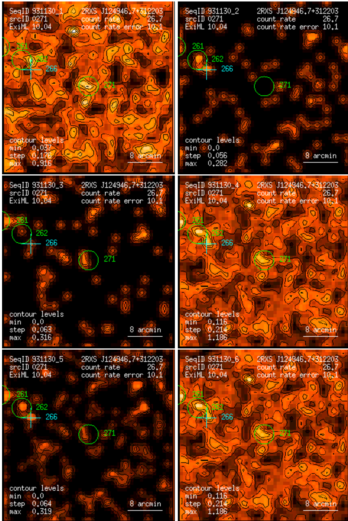
Figure 271: RASS 931130: detection 0271: band rate images, Gaussian filter: (1) PSPC channels 11 – 41, (2) 52 – 90, (3) 91 – 201, (4) 11 – 235, (5) 52 – 201, (6) 11 – 201. Broad band rates in counts/ks. Band rate contour levels in counts/ks/arcmin 2 .
