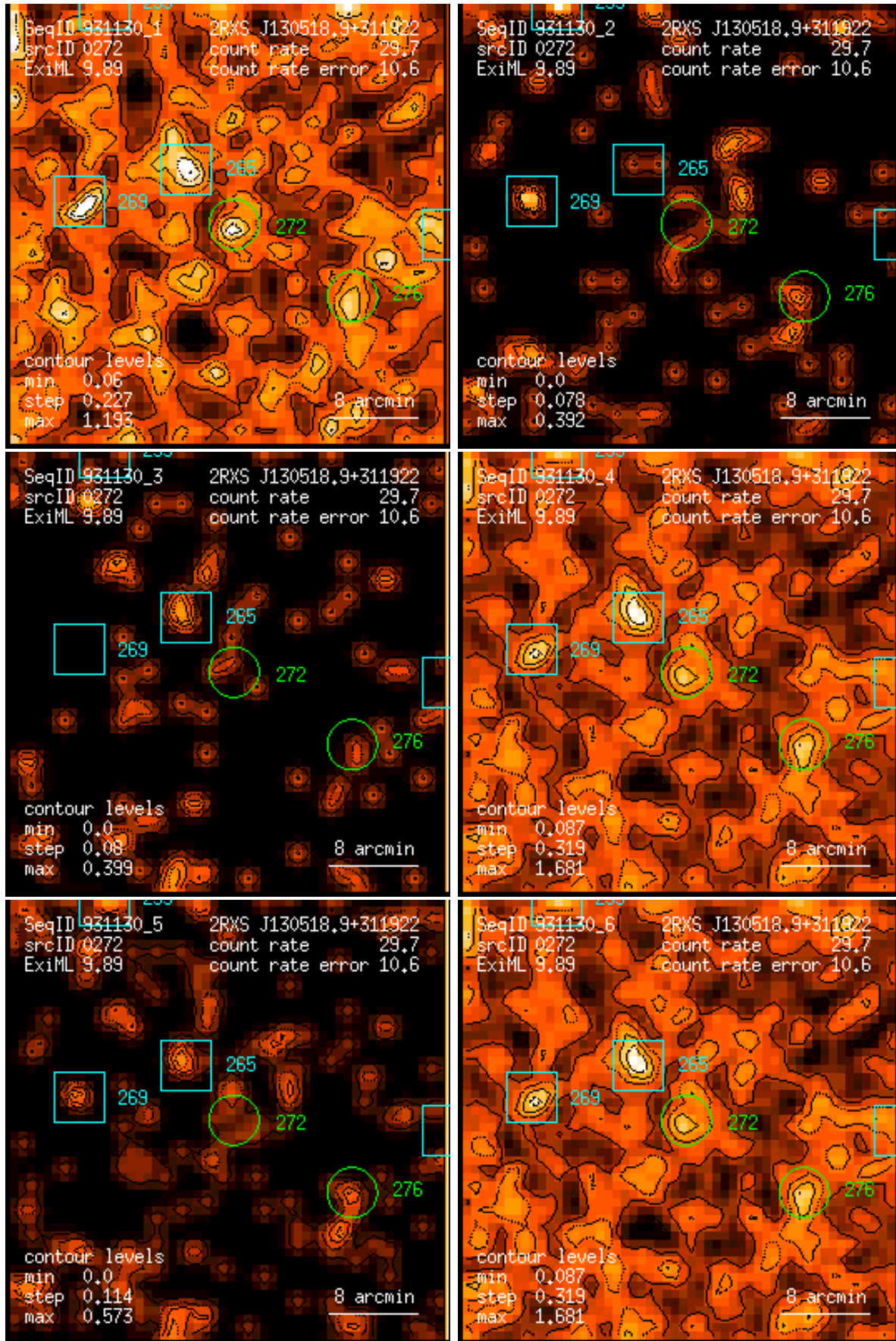
Figure 272: RASS 931130: detection 0272: band rate images, Gaussian filter: (1) PSPC channels 11 – 41, (2) 52 – 90, (3) 91 – 201, (4) 11 – 235, (5) 52 – 201, (6) 11 – 201. Broad band rates in counts/ks. Band rate contour levels in counts/ks/arcmin 2 .
