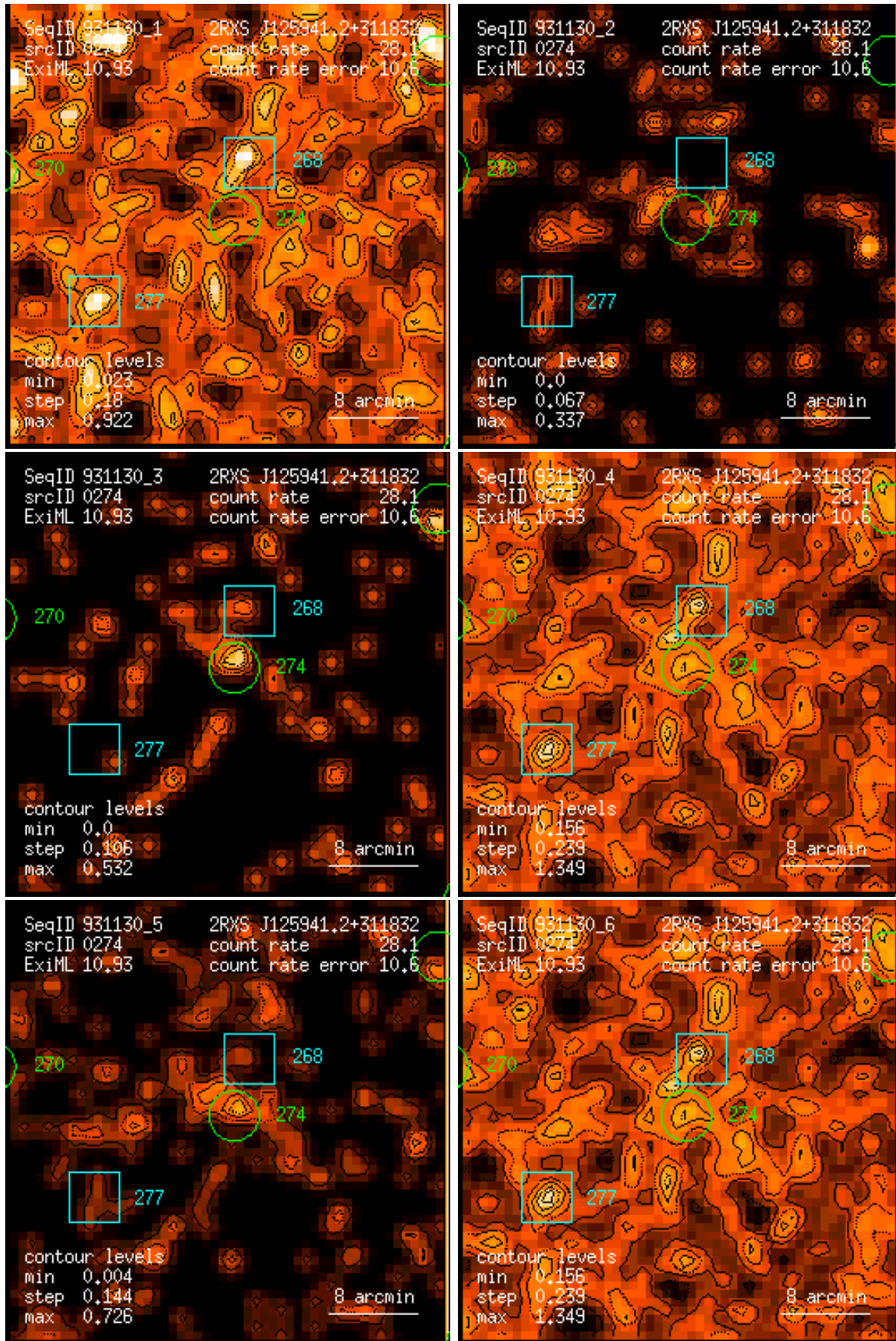
Figure 274: RASS 931130: detection 0274: band rate images, Gaussian filter: (1) PSPC channels 11 – 41, (2) 52 – 90, (3) 91 – 201, (4) 11 – 235, (5) 52 – 201, (6) 11 – 201. Broad band rates in counts/ks. Band rate contour levels in counts/ks/arcmin 2 .
