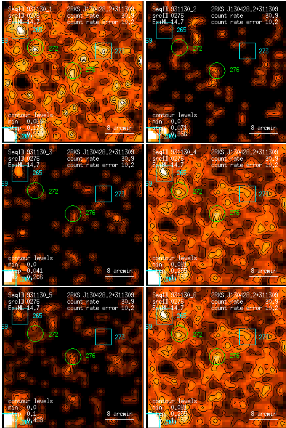
Figure 276: RASS 931130: detection 0276: band rate images, Gaussian filter: (1) PSPC channels 11 – 41, (2) 52 – 90, (3) 91 – 201, (4) 11 – 235, (5) 52 – 201, (6) 11 – 201. Broad band rates in counts/ks. Band rate contour levels in counts/ks/arcmin 2 .
