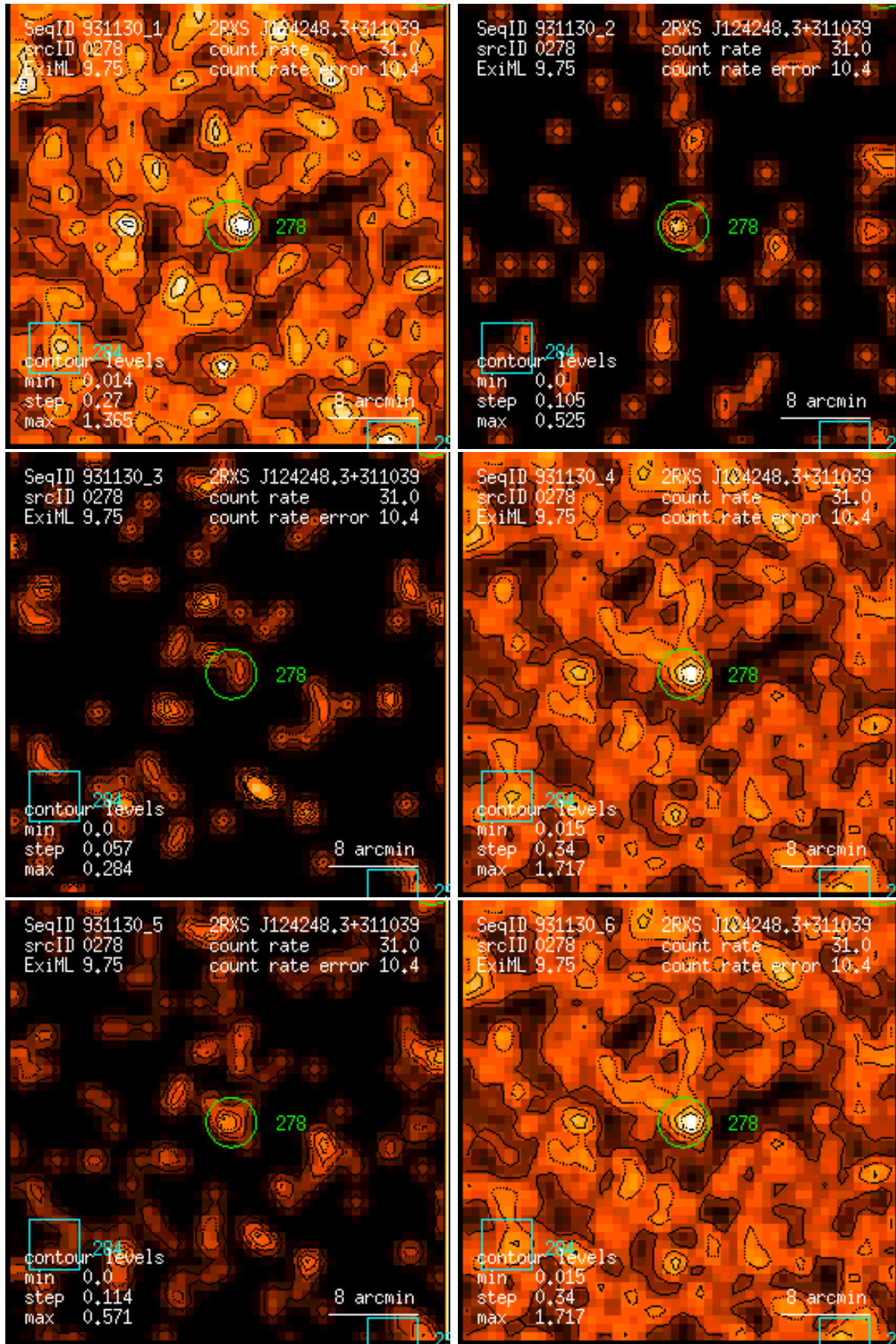
Figure 278: RASS 931130: detection 0278: band rate images, Gaussian filter: (1) PSPC channels 11 – 41, (2) 52 – 90, (3) 91 – 201, (4) 11 – 235, (5) 52 – 201, (6) 11 – 201. Broad band rates in counts/ks. Band rate contour levels in counts/ks/arcmin 2 .
