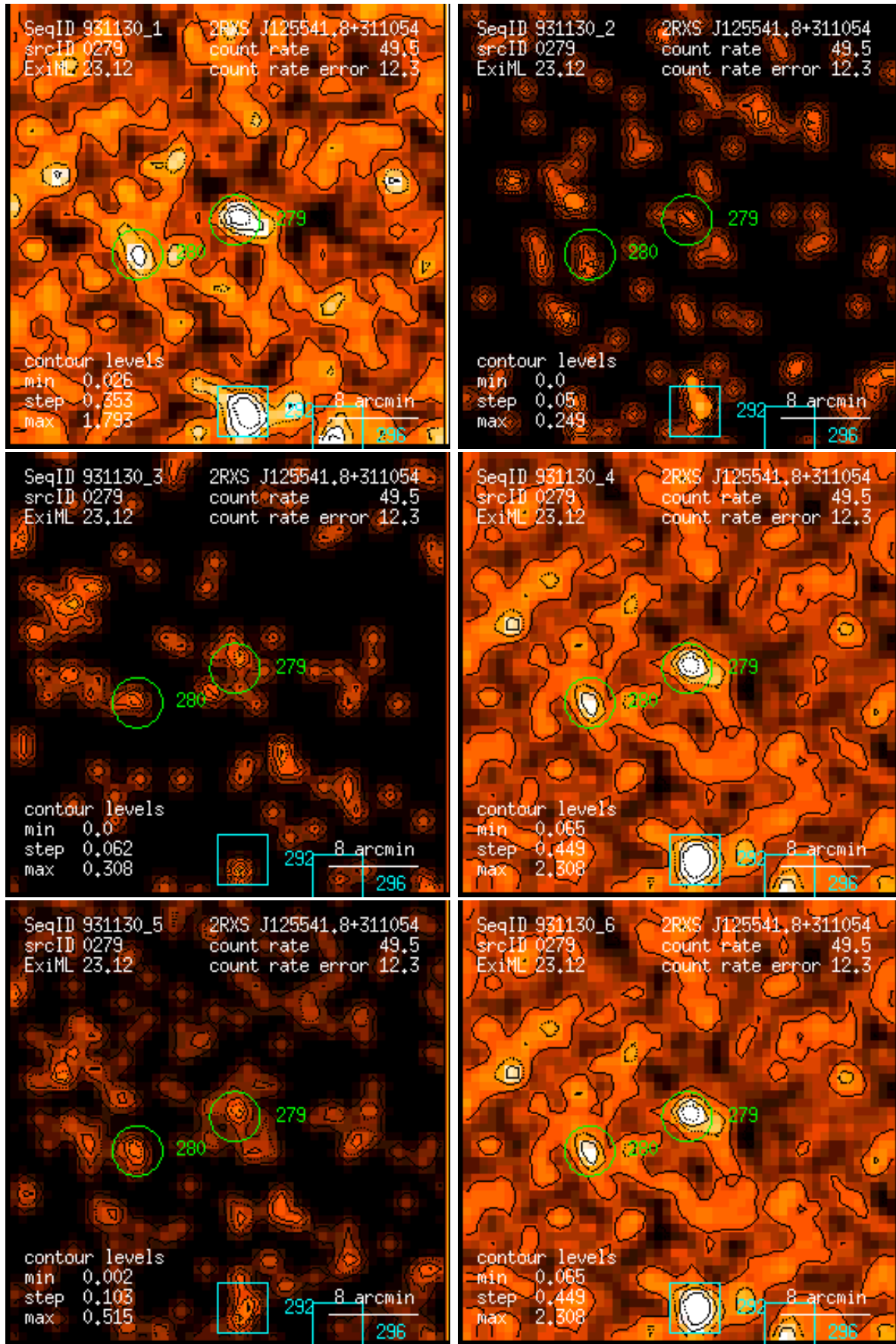
Figure 279: RASS 931130: detection 0279: band rate images, Gaussian filter: (1) PSPC channels 11 – 41, (2) 52 – 90, (3) 91 – 201, (4) 11 – 235, (5) 52 – 201, (6) 11 – 201. Broad band rates in counts/ks. Band rate contour levels in counts/ks/arcmin 2 .
