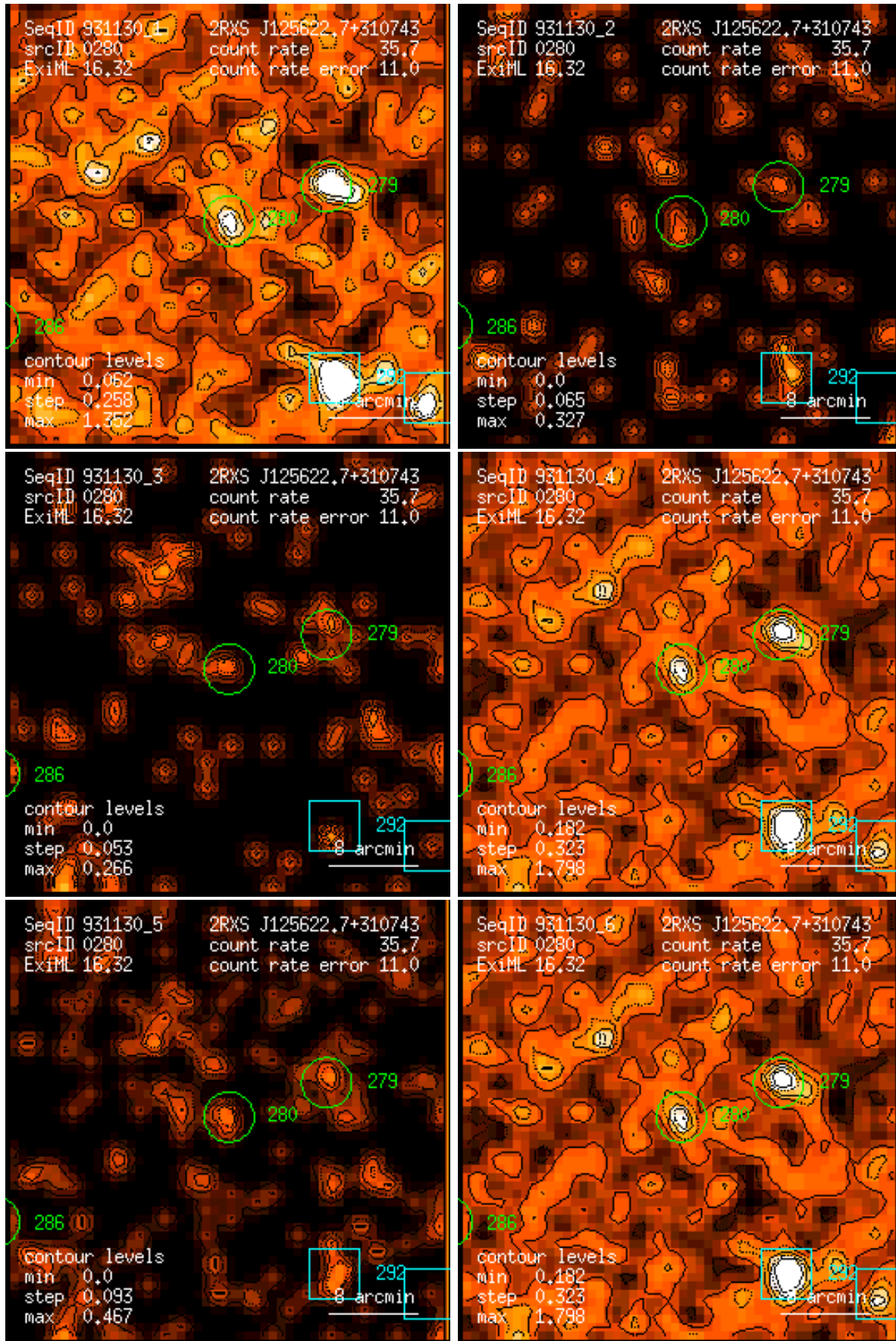
Figure 280: RASS 931130: detection 0280: band rate images, Gaussian filter: (1) PSPC channels 11 – 41, (2) 52 – 90, (3) 91 – 201, (4) 11 – 235, (5) 52 – 201, (6) 11 – 201. Broad band rates in counts/ks. Band rate contour levels in counts/ks/arcmin 2 .
