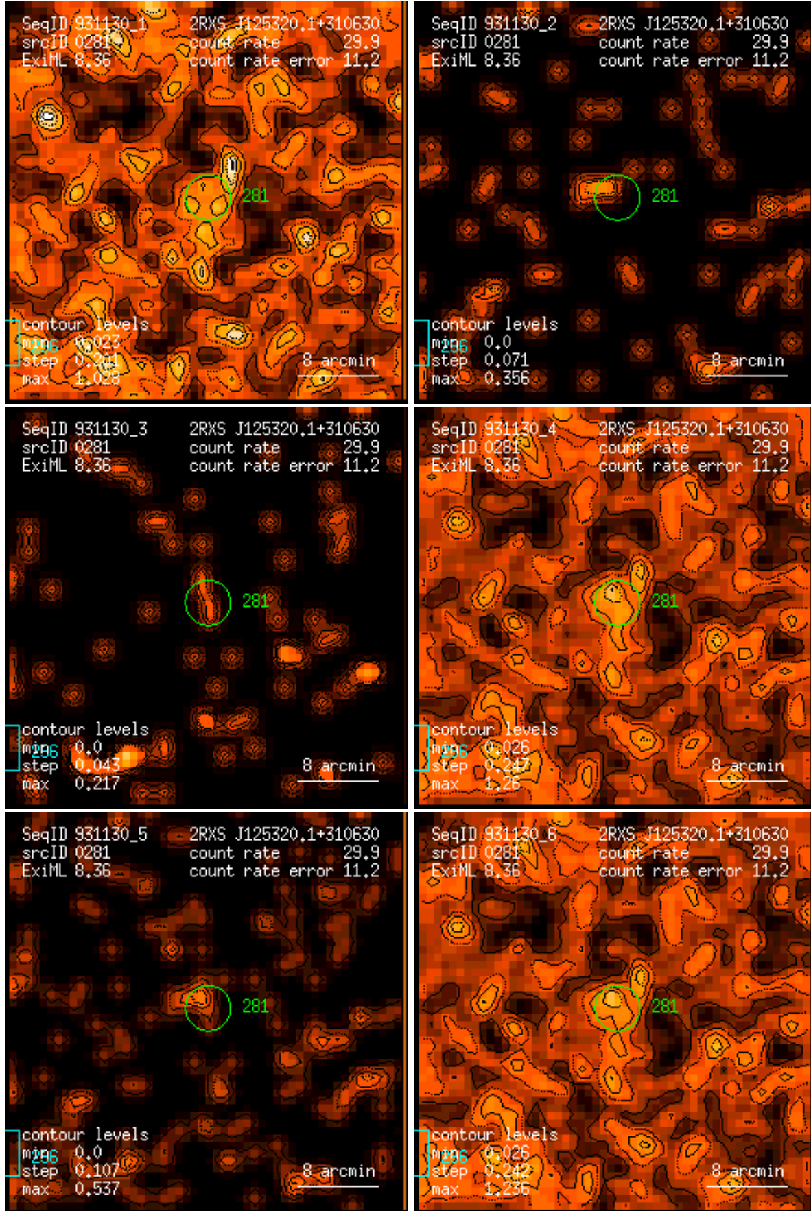
Figure 281: RASS 931130: detection 0281: band rate images, Gaussian filter: (1) PSPC channels 11 – 41, (2) 52 – 90, (3) 91 – 201, (4) 11 – 235, (5) 52 – 201, (6) 11 – 201. Broad band rates in counts/ks. Band rate contour levels in counts/ks/arcmin 2 .
