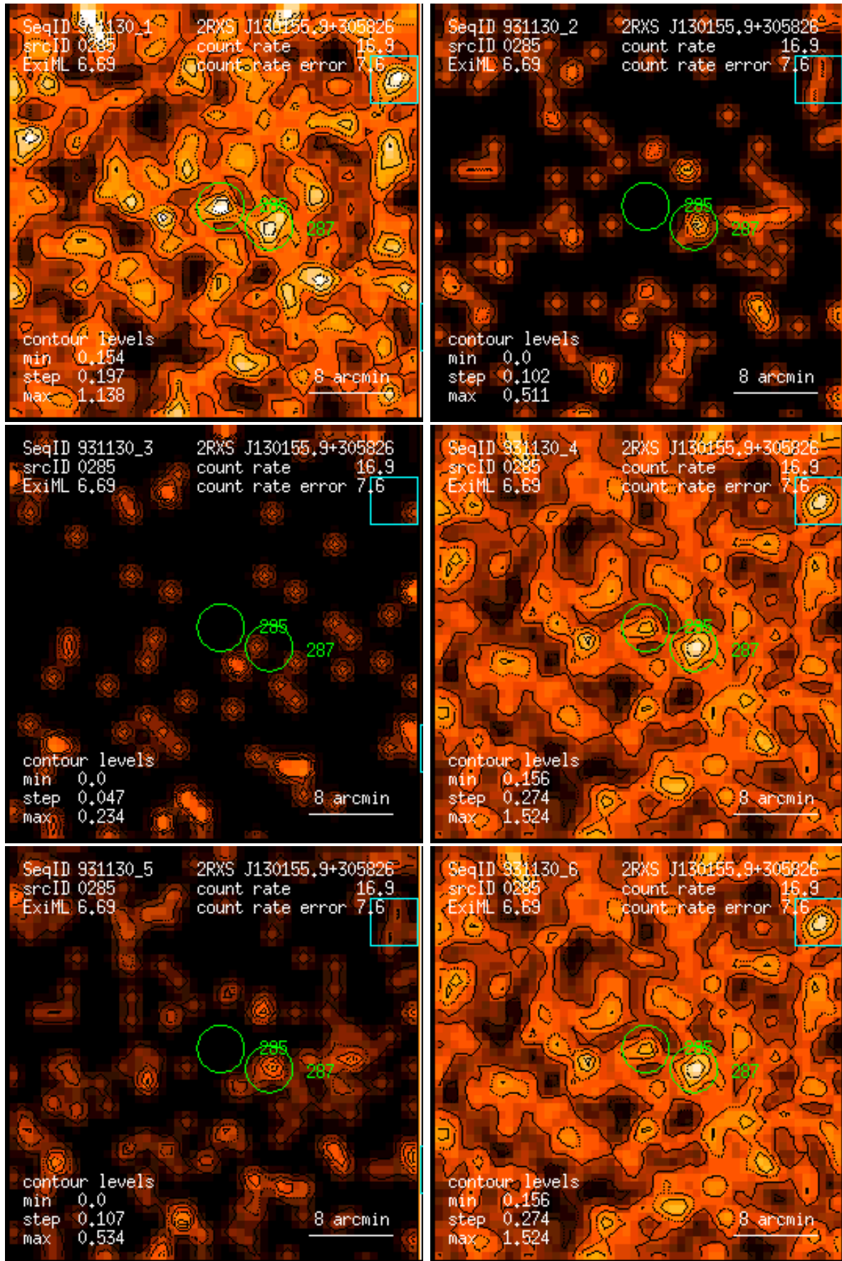
Figure 285: RASS 931130: detection 0285: band rate images, Gaussian filter: (1) PSPC channels 11 – 41, (2) 52 – 90, (3) 91 – 201, (4) 11 – 235, (5) 52 – 201, (6) 11 – 201. Broad band rates in counts/ks. Band rate contour levels in counts/ks/arcmin 2 .
